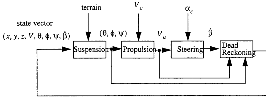
Figure 5: Feedforward simulator.
