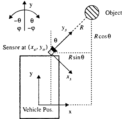
Figure 5: Sensor to object transformation.
