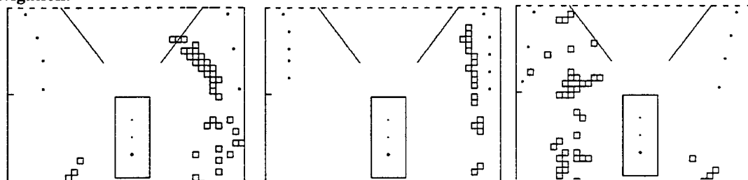
(c) Display of the local traversability map at the locations marked by arrows in (a) and (b). Only the portion of the map in the immediate vicinity of the vehicle is displayed here. The vehicle is depicted by a rectangle. The untraversable regions are shown as squares.
