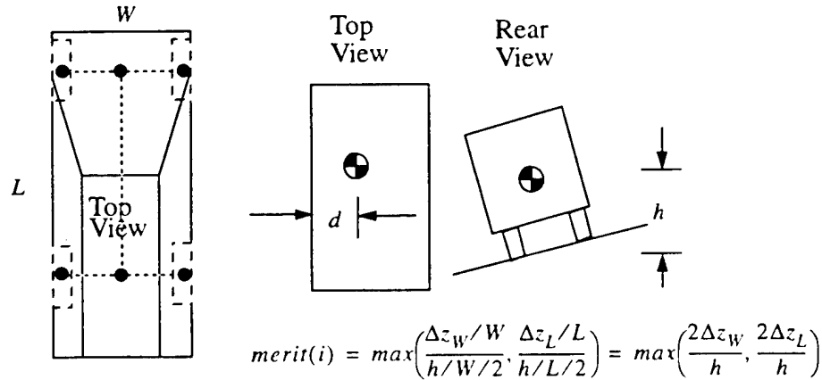
Figure 13: Static stability.
