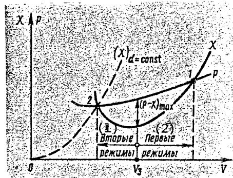
Figure 2. Boundary Between Primary and Secondary Flight Phases
