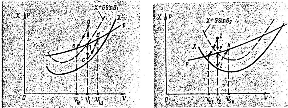
Figure 4, 5. Dependence of Thrust and Drag on Velocity During Transition From One Flight Trajectory to Another
