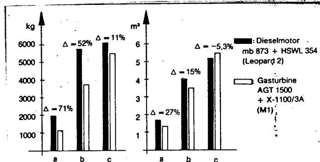
Figure 56. Comparison of Leopard 2 and M1 engine weight and volume: (a) engine or gas turbine separately, (b) complete powerplant, and fuel reserve for circa 450 km road travel
