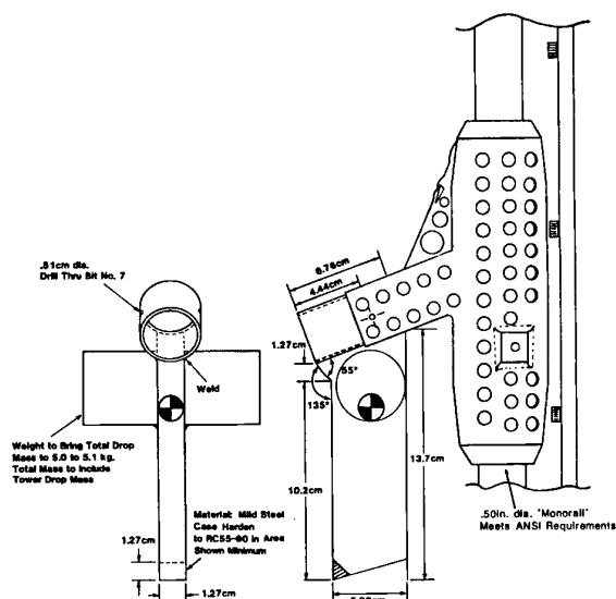
Figure 18. Helmet tear test penetrator.
