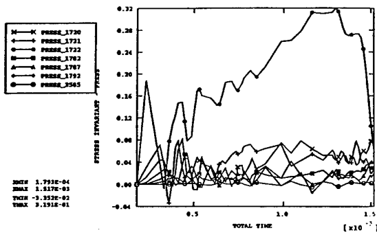
Figure 17 The results from Abaqus: Pressure time history of the selected elements which are located in the cross section of the brain where the impactor hits. The elements are labeled in sequence as (A)1722-the impact surface, (B)1721, (C)1720, (D)1782, (E)1787, (F)1792, and (G)3585-the deep center of the brain. Pressure is in MPa and time is in seconds.
