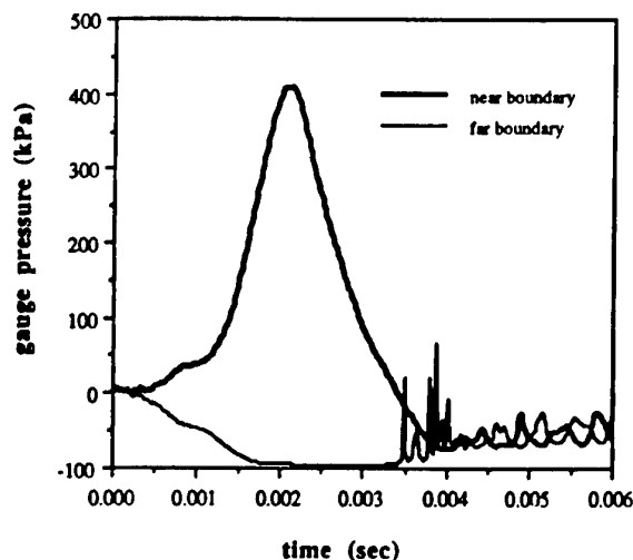
Figure 7: High acceleration pressure response with 20-g neck acceleration.
