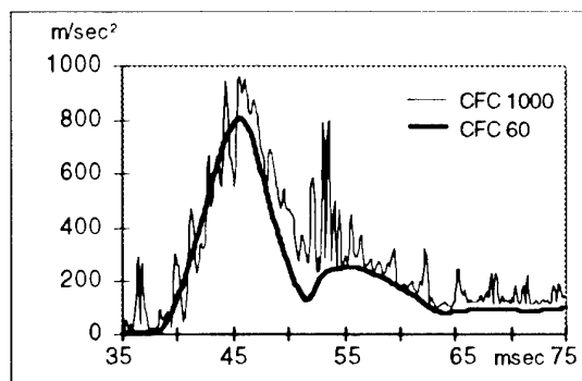
Fig. 3: Resultant acceleration time-history at the head c.g. of a padded occipital head impact using CFC 1000 and CFC 60.
