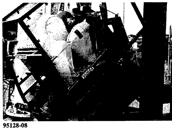
Figure 11. AH-64 Apache helicopter crewstation mock-up mounted in the dynamic test facility.
