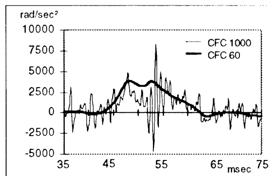
Fig. 4: Head rotational acceleration-time history around the y-axis of a padded occipital head impact using CFC 1000 and CFC 60.
