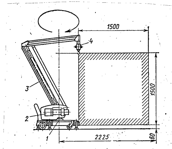
Figure 8. MP-100 Electromechanical Loading Manipulator: 1--carriage; 2--power drive; 3--lever mechanism; 4--freight unit
