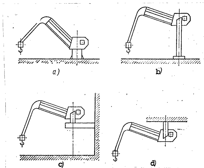
Figure 9. Versions of MP-100 Loading Manipulator: a--installation on floor on base; b--installation on floor on column; c--attachment to wall on bracket; d--attachment to ceiling
