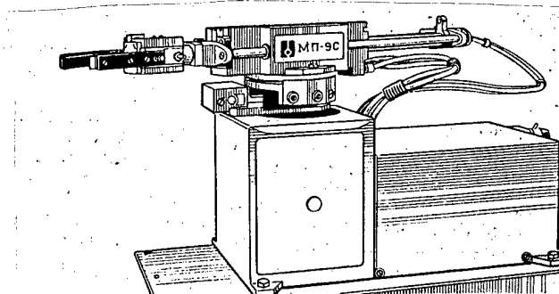
Figure 2. MP-9S Automatic Manipulator
