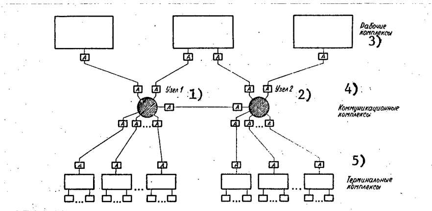
Figure 3. Physical Structure of Experimental Computer Network (EVS)
