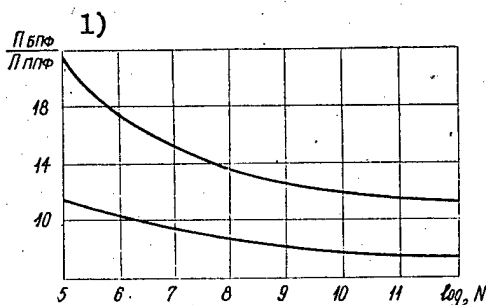
Figure 2. Functions for Reduction of the Number of Whole-Number Multiplication Operations for the Digital Fourier Transform Algorithm While Using Various Orthogonal Periodic Functions, as Compared with the Fast Fourier Transform Algorithm: a--algorithms when using system 1; b--algorithms when using system 2
