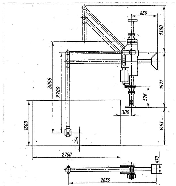
Figure 10. KSh-63 Manipulator
