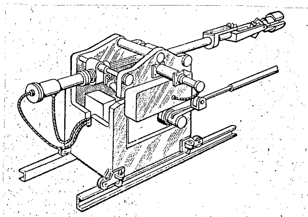
Figure 5. Manipulator for Forging Rolls
