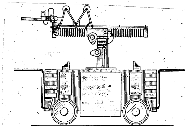
Figure 1. MP-12 Automatic Manipulator
