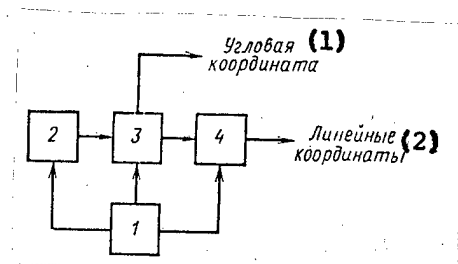
Figure 12. Block Diagram of Correlation Vision (KZ): 1--control unit of operating modes; 2--video camera; 3--optical image comparison unit; 4--coordinate recalculation unit
