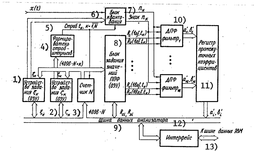
Figure 3. Structural Diagram of Spectrum Analyzer
