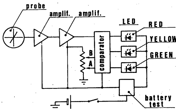
Fig. 4 - Block diagram of the RF Hazard Monitor.
