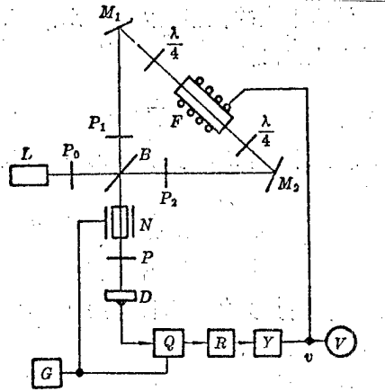
Fig. 1. Operating principles of device.
