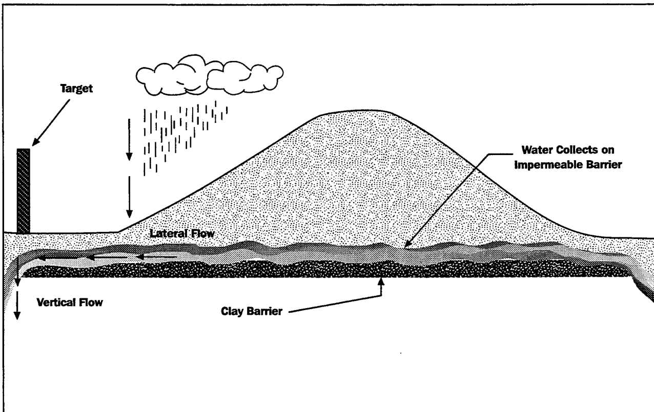
FIGURE 6 PROBLEMS ASSOCIATED WITH CLAY LAYERS AND BARRIERS
