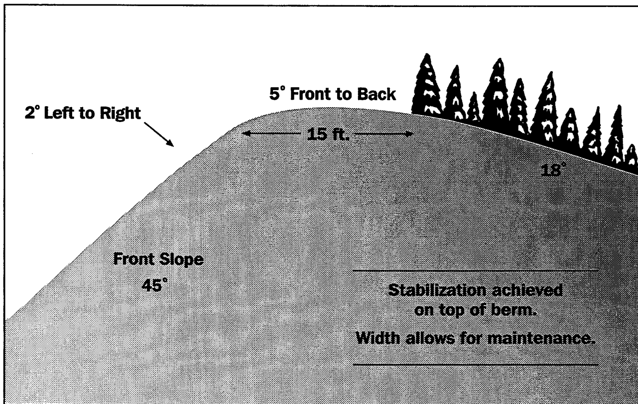
FIGURE 7 CONTOURING BACKSTOPS TO CONTROL EROSION
