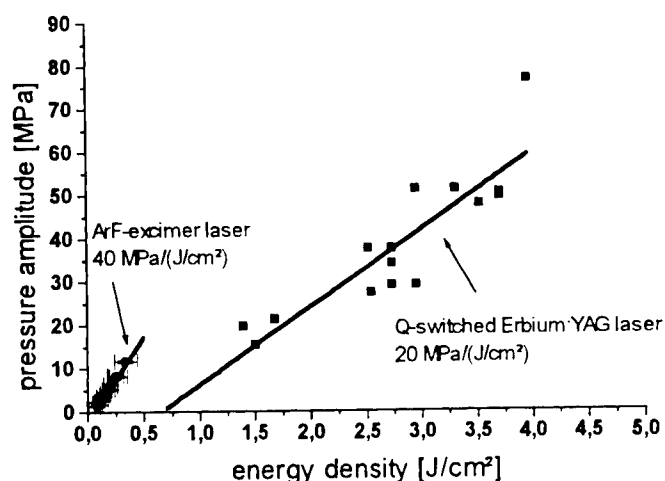
Fig. 1: Laser induced pressure amplitudes in dependence on the energy density for an ArF-excimer laser and a Q-switched Erbium:YAG laser. The laser pulse duration of the ArF-excimer laser was 20 nsec and 300 nsec for the Q-switched Erbium:YAG laser. A numerical linear fit to the data's results in an slope factor of 40 \text{ MPa/(J/cm}^2) for the ArF-excimer laser and 20 \text{ MPa/(J/cm}^2) for the Q-switched Erbium:YAG laser at energy densities above the ablation threshold ( F > F_{th} ). The pressure amplitudes were measured by a piezoelectric detector consisting of an PVDF-film.
