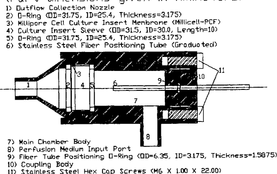
Figure 1 - Assembled Chamber View (Part dimensions given in millimeters)
