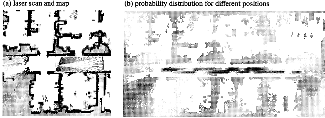
Figure 5: Probabilistic model of perception: (a) Laser range scan, projected into a previously acquired map. (b) The probability P(o \mid \xi) , evaluated for all positions \xi and projected into the map (shown in grey). The darker a position, the larger P(o \mid \xi) .
