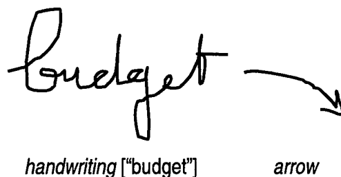
Figure 10. Gesture/Handwriting Combination
