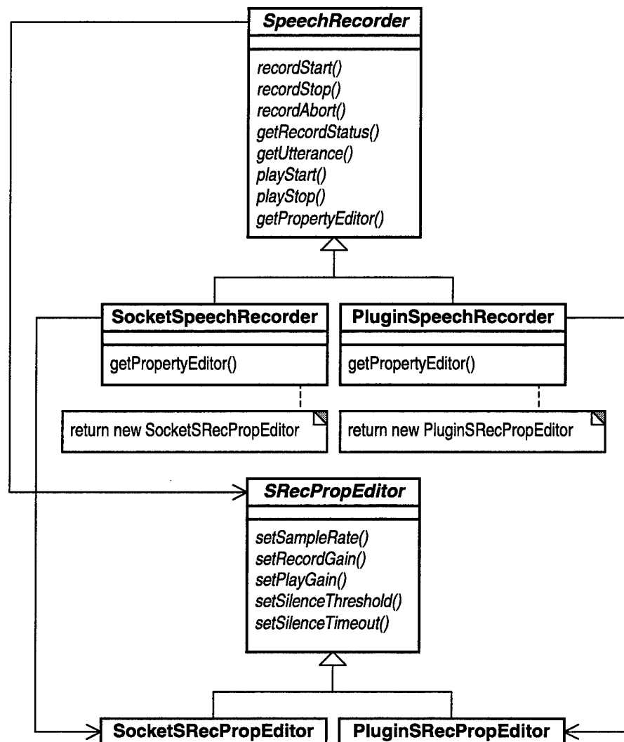
Figure 11. SpeechRecorder Interface
