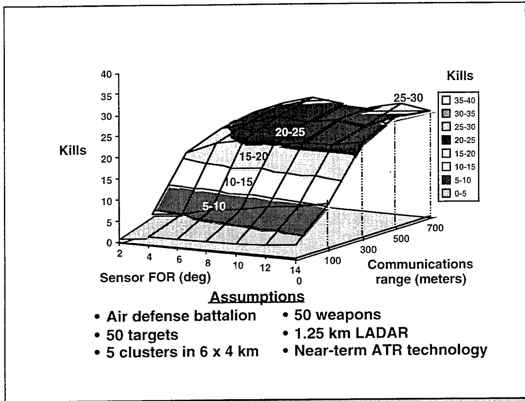
Figure 3.13—Improved Communication Enhances Effectiveness More Than Sensor Field of Regard for Large Targets
