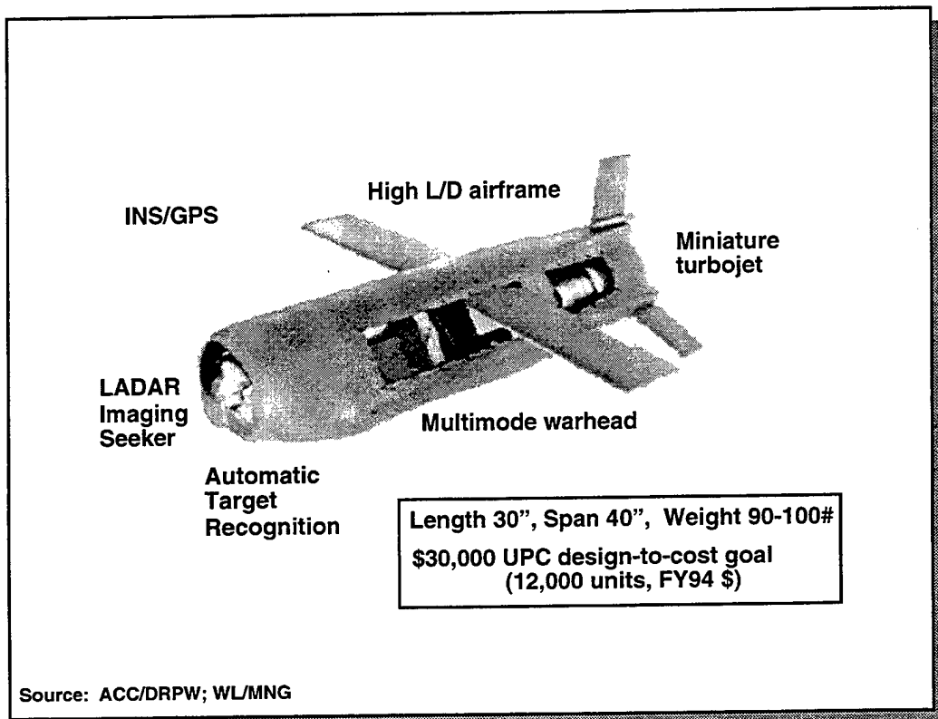
Figure 3.6—LOCAAS Configuration
