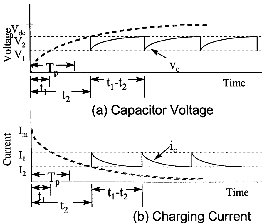
Figure 13 : Waveforms
