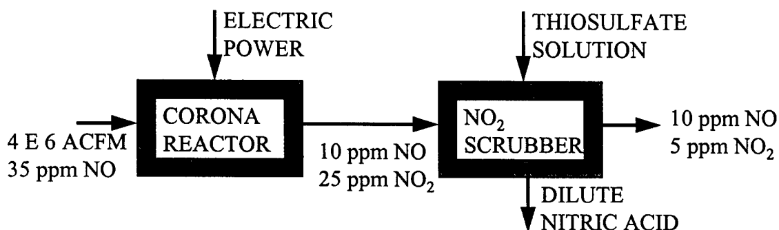
Figure 11 : Flow Diagram for NO x Removal Process
