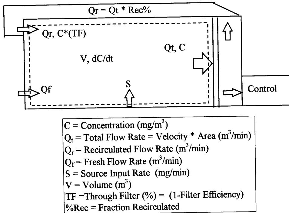
Figure 3-1 Airflow Diagram
