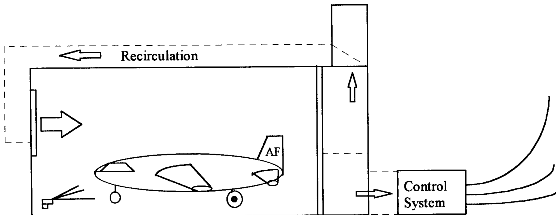
Figure 1-1 Recirculation Concept
