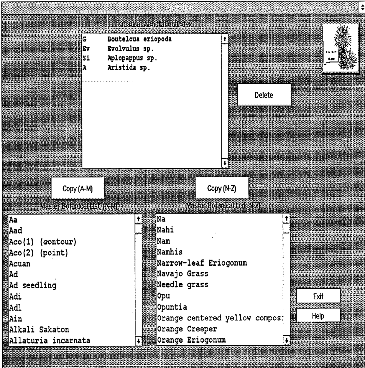
Figure 3. Annotation GUI
