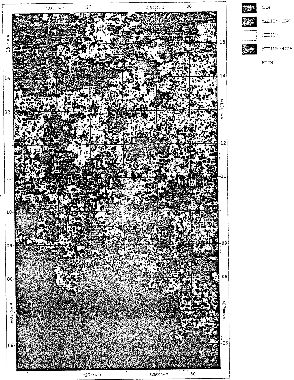
SOIL-ADJUSTED VEGETATION INDEX 9 June 1993 SPOTVIEW Imagery
