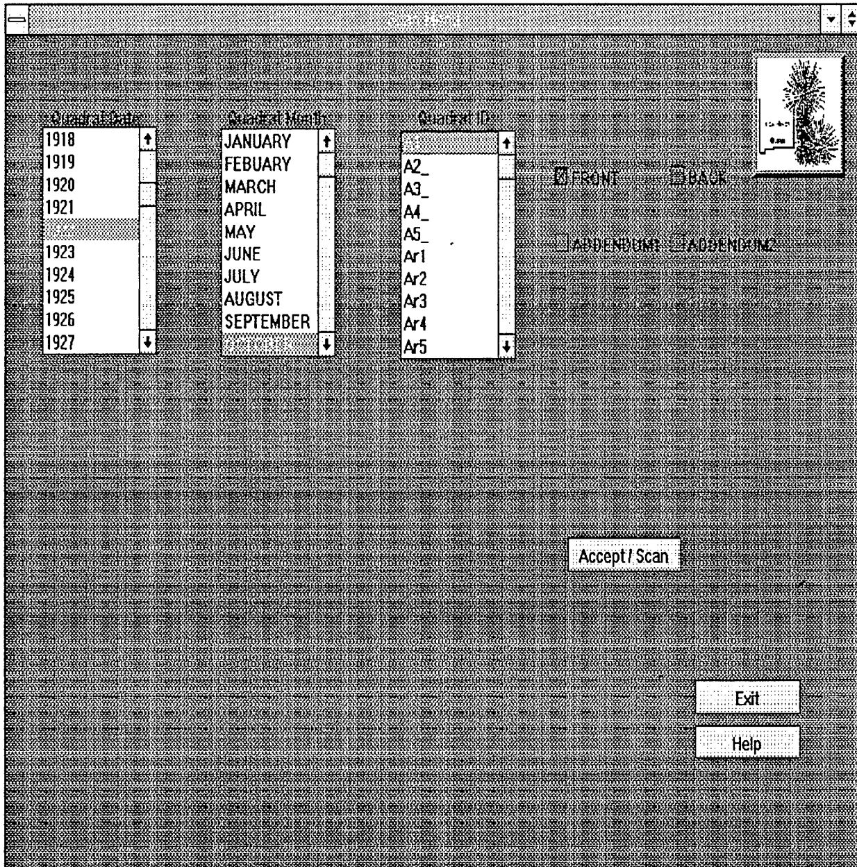
Figure 2. Scan GUI
