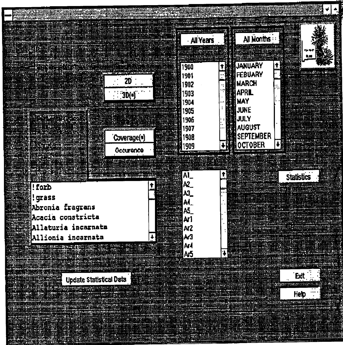
Figure 8. Statistical GUI
