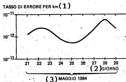
Fig 2 - Recordings of daily error rate per km on Mestre-Padua-Mestre link, with loop at Padua (64 km).
