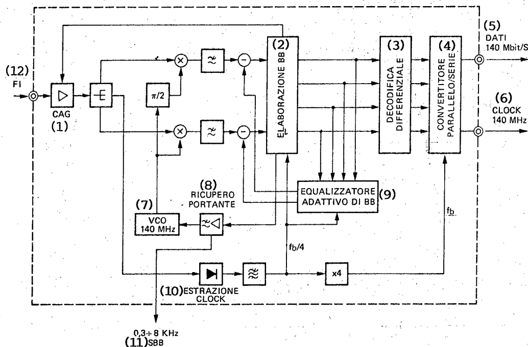
Fig 16 - Simplified block diagram of demodulator.
