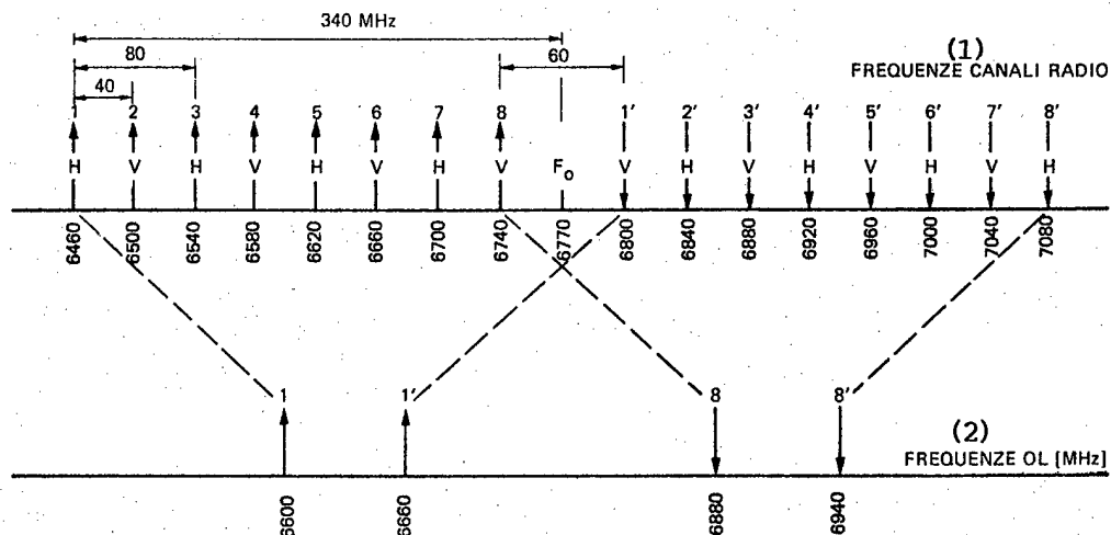
Fig 4 - RF channeling and positioning of local oscillators.
