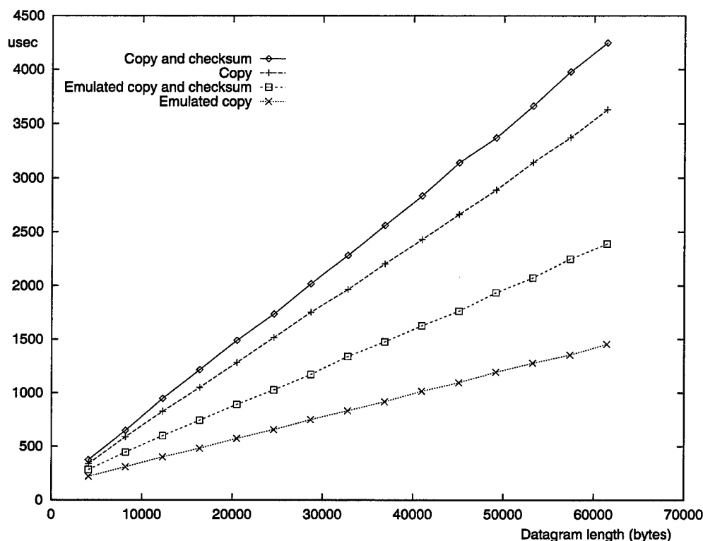
Figure 8.6: Single-packet end-to-end latency with or without checksumming. Emulated copy is cheaper than copy even if the host processor also has to read the data for checksumming.
