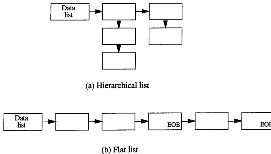
Figure 6.7: Data buffer representation alternatives.
