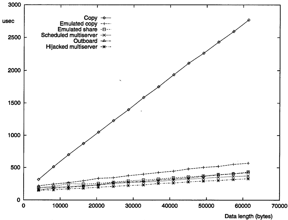
Figure 12.4: I/O processing time ( t_{I/O} ) of data transfer from Cyclone board to ATM network.
