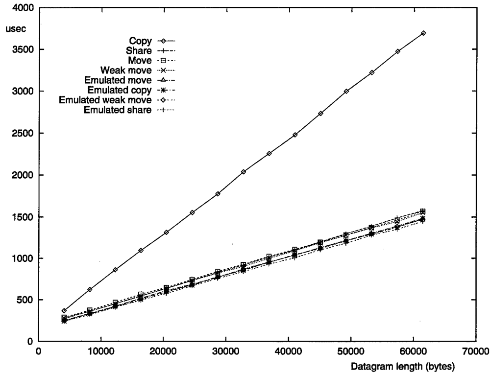
Figure 8.3: Single-packet end-to-end latency with client-aligned pooled in-host buffering. If there is alignment, native-mode schemes other than copy give performances similar to those of migrant-mode schemes.
