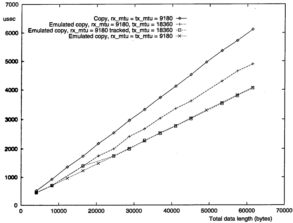
Figure 8.8: Multiple-packet end-to-end latency with early demultiplexing at 155 Mbps. Copying is avoided regardless of client input buffer alignment and MTU. The MTU can be quickly estimated by MTU tracking.
