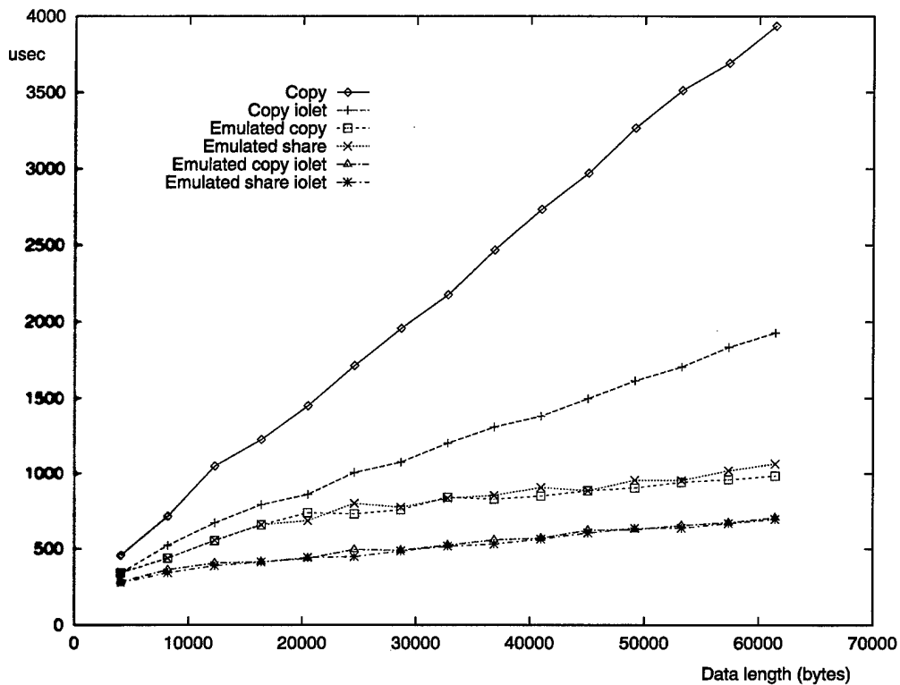
Figure 12.6: I/O processing time ( t_{I/O} ) to output the same client data to Cyclone board and ATM network.
