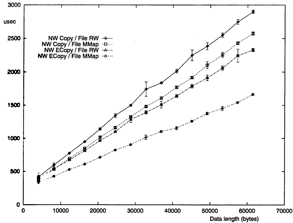
Figure 10.1: Fetch response time in the case of a hit.
