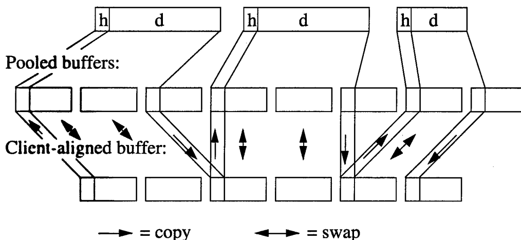
Figure 6.1: Copy avoidance with pooled in-host buffering and client-aligned buffering.
