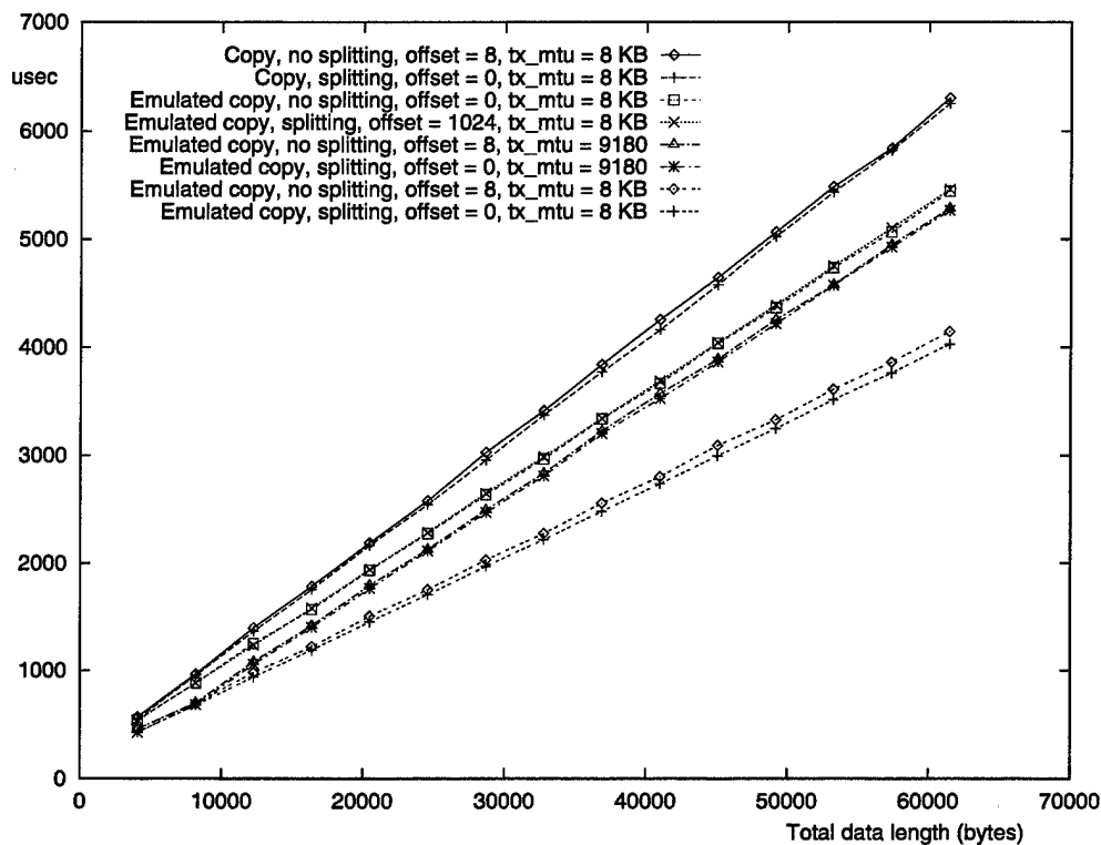
Figure 8.7: Multiple-packet end-to-end latency with pooled in-host buffering at 155 Mbps. The performance of client-aligned buffering is not substantially affected by the presence or absence of header/data splitting.
