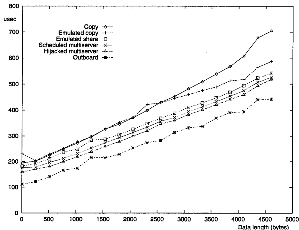
Figure 12.2: Total latency of short data transfer from Cyclone board to ATM network on otherwise idle system.
