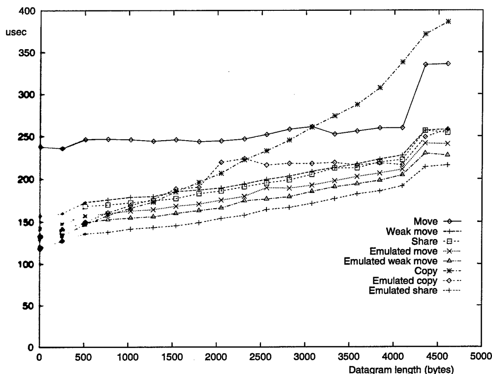
Figure 8.2: Single-packet end-to-end latency for short data, using early demultiplexing. Using reverse copyout, emulated copy avoids copying more than about half a page.
