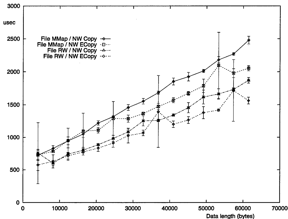
Figure 10.7: Store I/O processing time in case of a miss.
