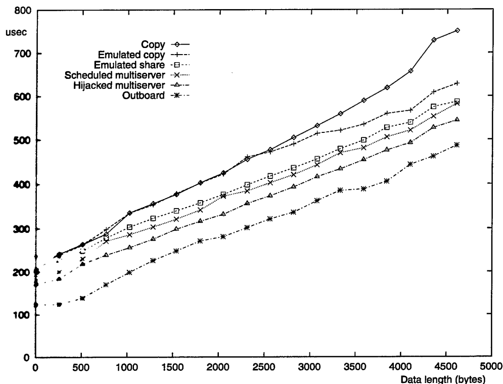
Figure 12.3: Total latency of short data transfer from Cyclone board to ATM network with ten concurrent compute-bound processes.
