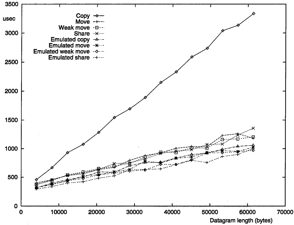
Figure 8.5: I/O processing time ( t_{I/O} ) with early demultiplexing. I/O with the copy scheme leaves much less CPU time available for client processing.
