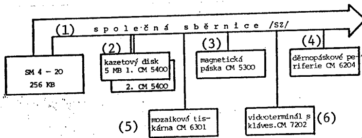
Figure 2. Configuration of the SM 4-20 minicomputer.
