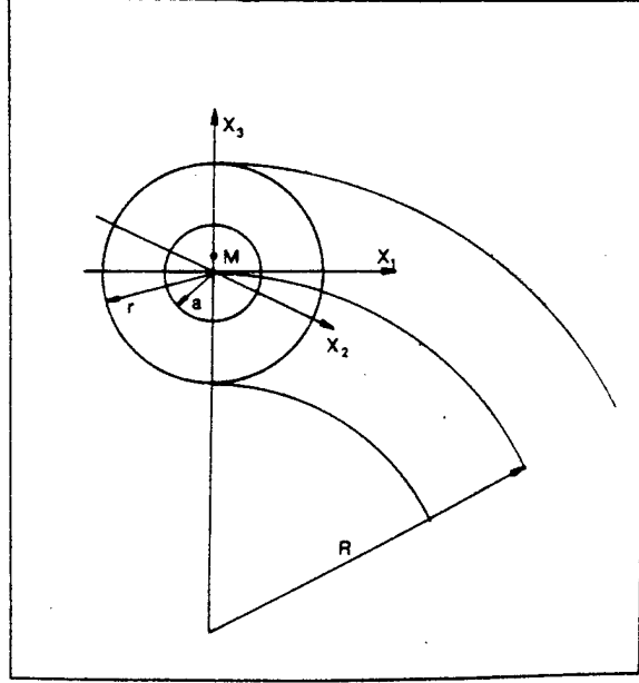
Fig. 4 - Fiber bending schematics; the maximum of the electric field distribution is displaced along the x_3 -axis to point M (see text).
