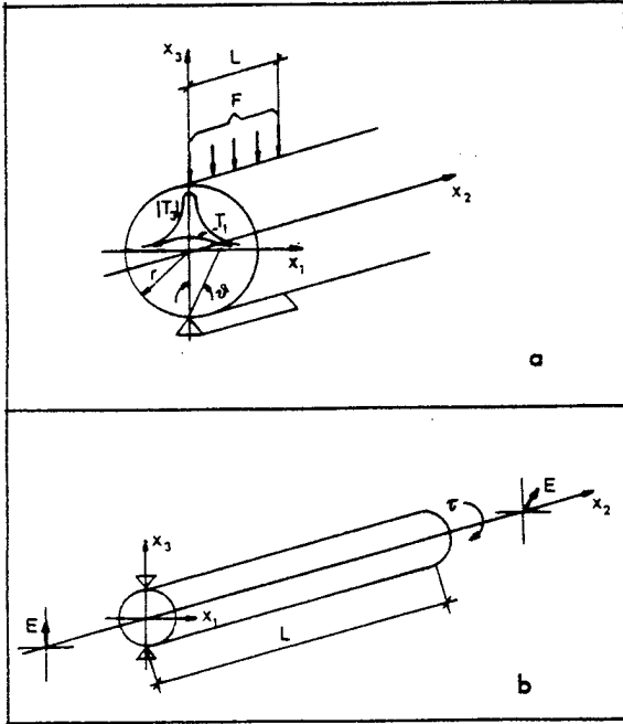
Fig. 1a) - Compression of an optical fibre by a force F . The strain distribution T_3 and T_1 are also shown.
