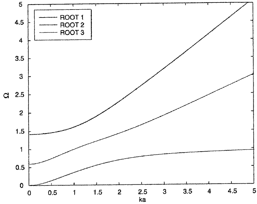
Figure 10. Frequencies for the n = 1 case.
