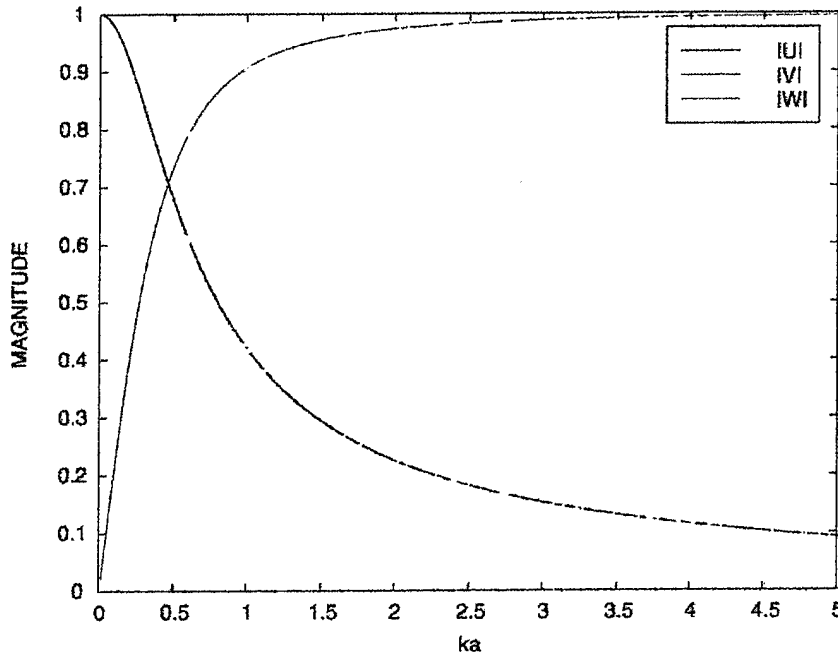
Figure 9. Displacements for root 3 of the n = 0 case.
