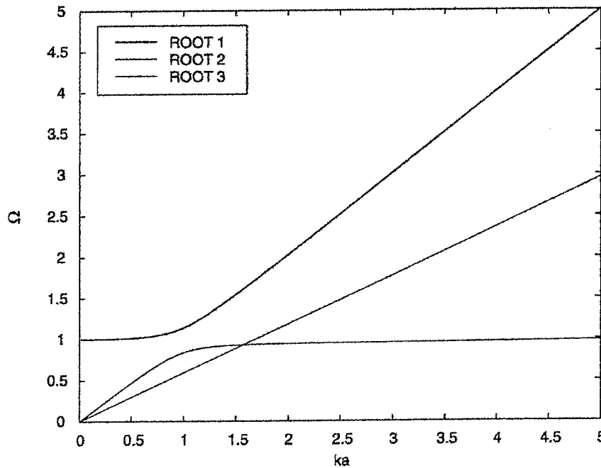
Figure 5. Frequencies for the n = 0 case.
