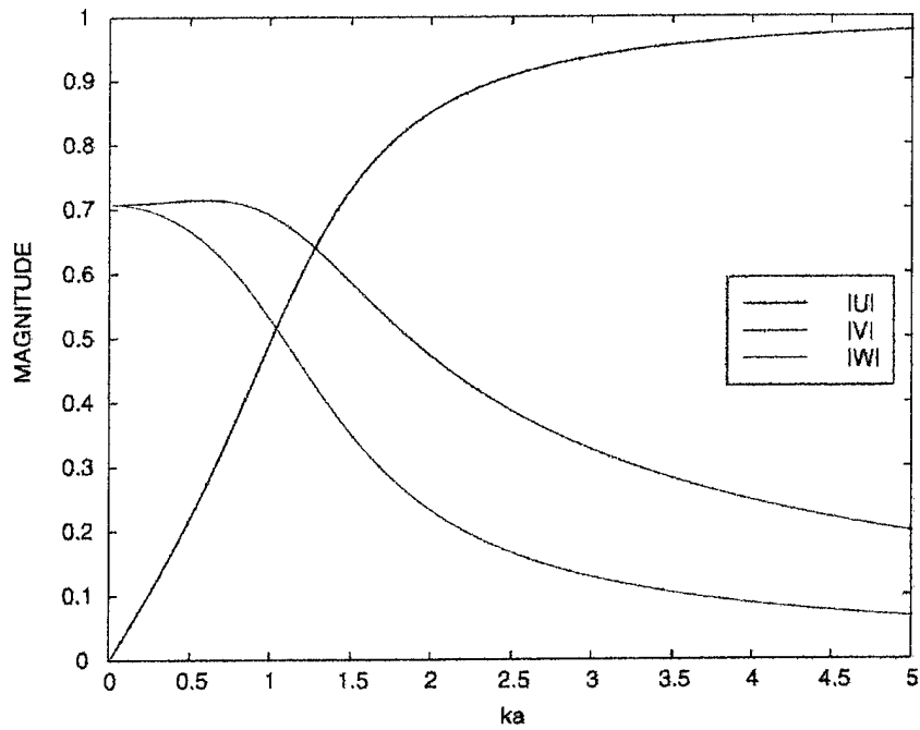
Figure 12. Displacements for root 1 of the n = 1 case.
