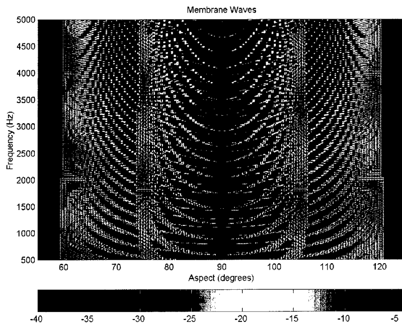
Figure 24. Predicted response over a wider bandwidth.
