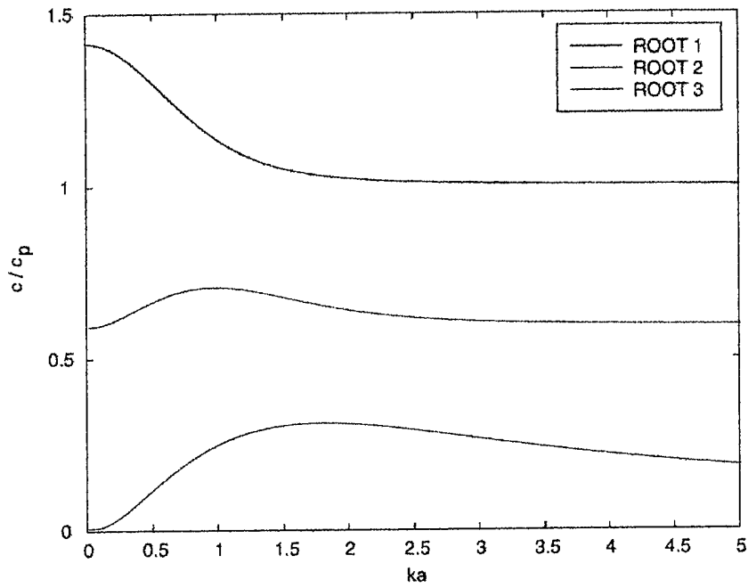
Figure 11. Phase velocities for the n = 1 case.
