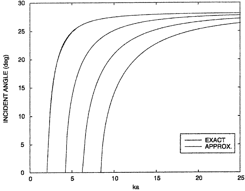
Figure 22. Comparison of approximate and "exact" solution for shear modes.
