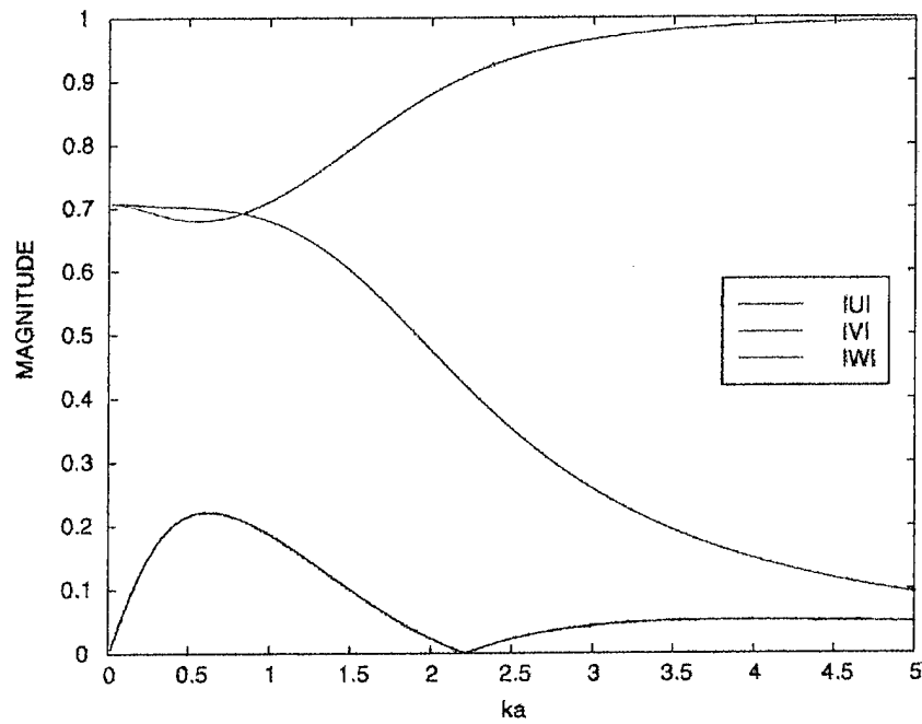
Figure 13. Displacements for root 2 of the n = 1 case.
