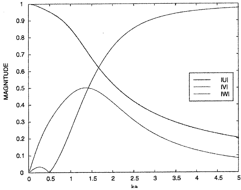
Figure 14. Displacements for root 3 of the n = 1 case.
