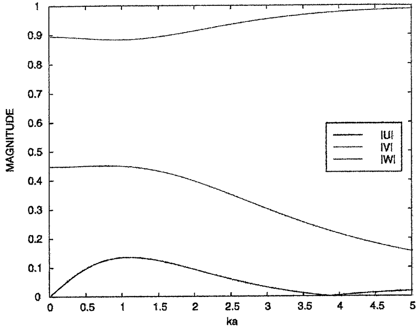
Figure 18. Displacements for root 2 of the n = 2 case.
