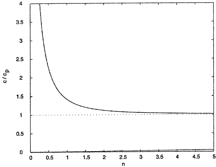
Figure 3. Example of dispersion curves for z-independent motion.
