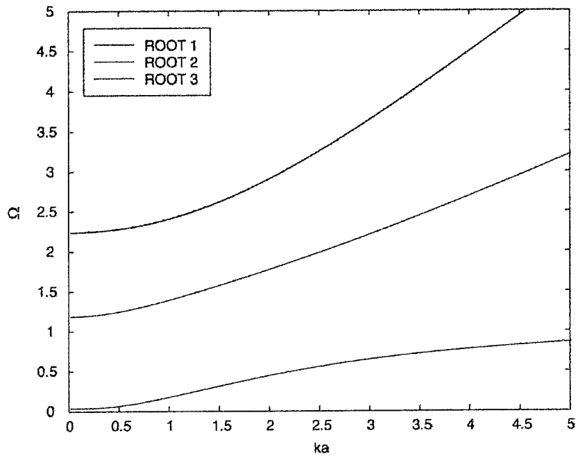
Figure 15. Frequencies for the n = 2 case.
