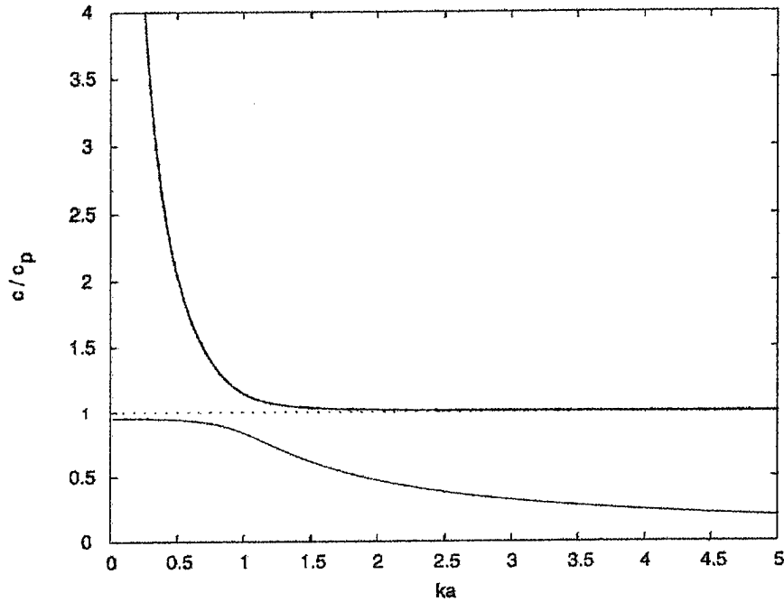
Figure 1. Example of dispersion curves for \theta -independent motion.
