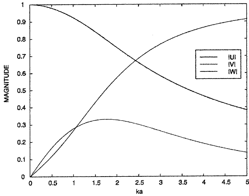
Figure 19. Displacements for root 3 of the n = 2 case.
