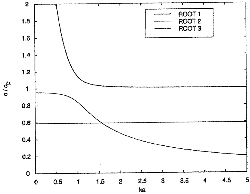
Figure 6. Phase velocities for the n = 0 case.
