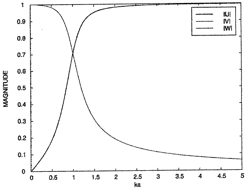
Figure 7. Displacements for root 1 of the n = 0 case.
