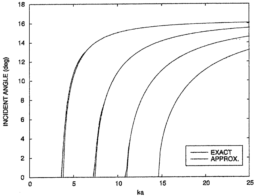
Figure 21. Comparison of approximate and "exact" solution for compressional modes.
