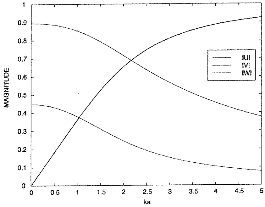
Figure 17. Displacements for root 1 of the n = 2 case.
