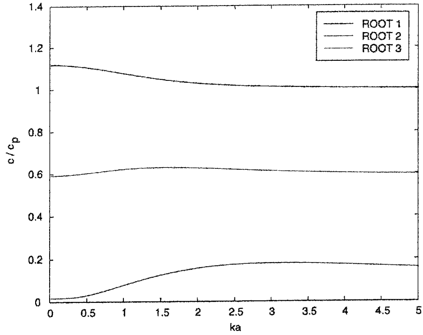
Figure 16. Phase velocities for the n = 2 case.
