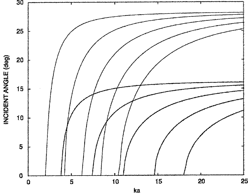
Figure 20. Example of dispersion curves as functions of frequency and incident angle.
