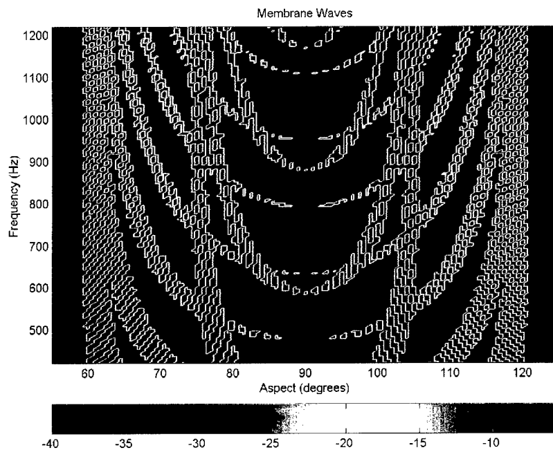
Figure 23. Predicted response for the example given by Rumerman (1993).
