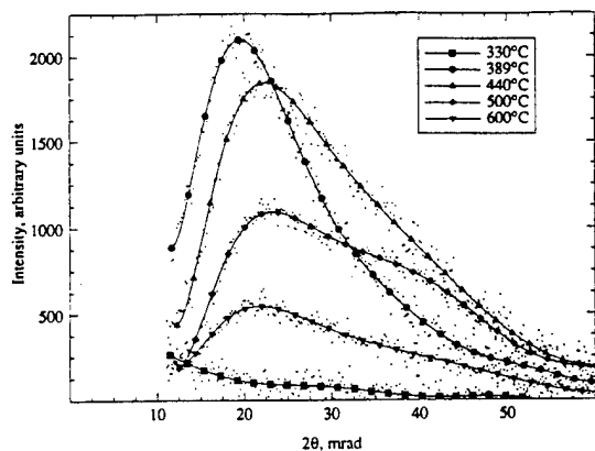
Fig. 18. SAXS curves of SAF stabilized in inert atmospheres at constant length and to high temperatures (argon, 1^{\circ}\text{C min}^{-1} ).
