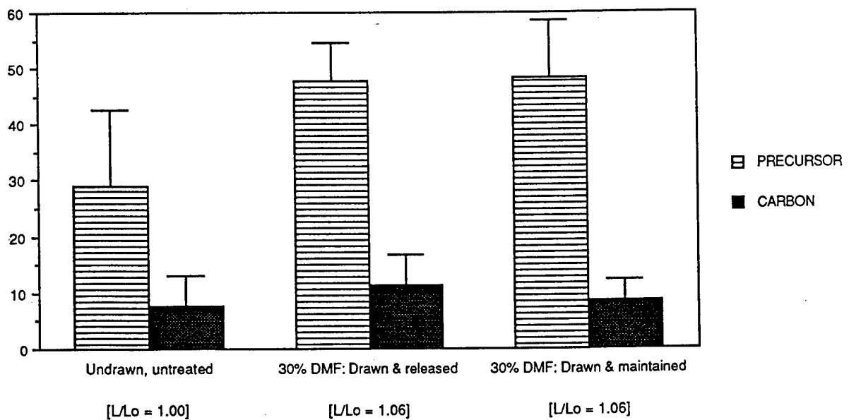
Toughness (MPa)
