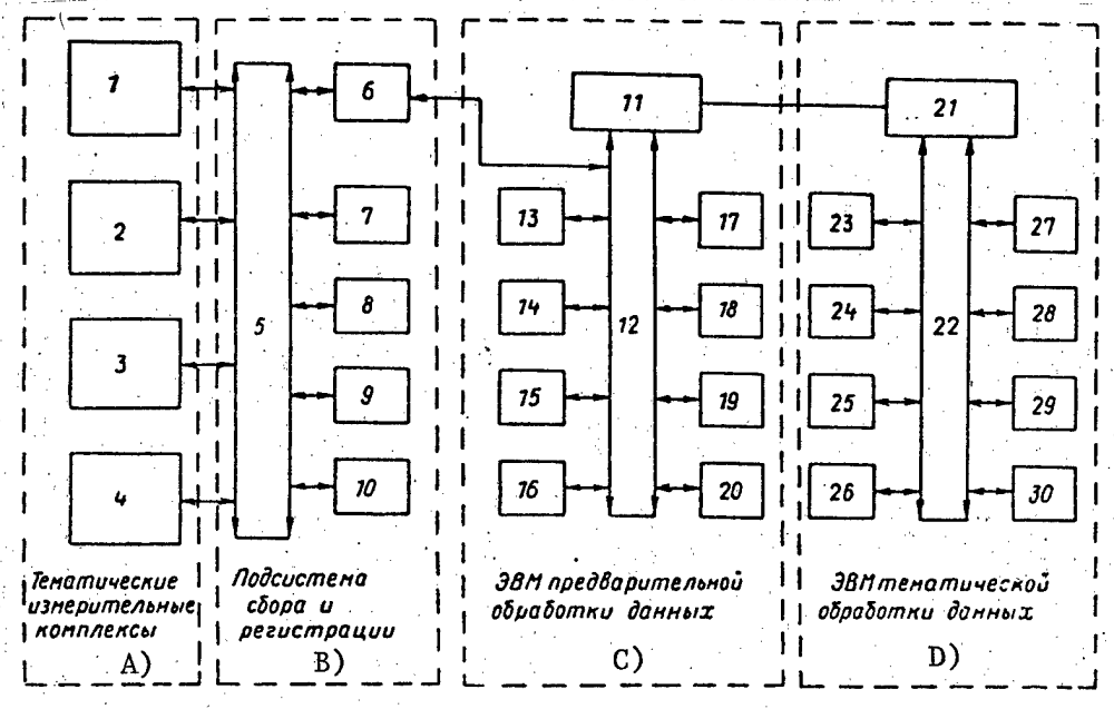
Fig. 1. Example of standard structure of shipboard system for automating experiment. 1, 2, 3, 4) hydrophysical, hydrochemical, geophysical, meteorological specialized measurement complexes respectively; 5) nonmachine line; 6) controller; 7) display; 8) cassette unit for storage on magnetic tape; 9) facsimile recorder; 10) oscillograph; 11, 21) central processor; 12, 22) machine line; 13, 27) analog-digital printout unit; 14) monitor; 15) curve plotter; 16) quasigraphic display; 17, 25) photoreadout; 18) puncher; 19, 30) unit for storage on magnetic disk; 20, 29) unit for storage on magnetic tape; 23) unit for input of graphic information; 24) precise curve plotter; 26) graphic display with unit for producing hard copy; 28) operator's display.
