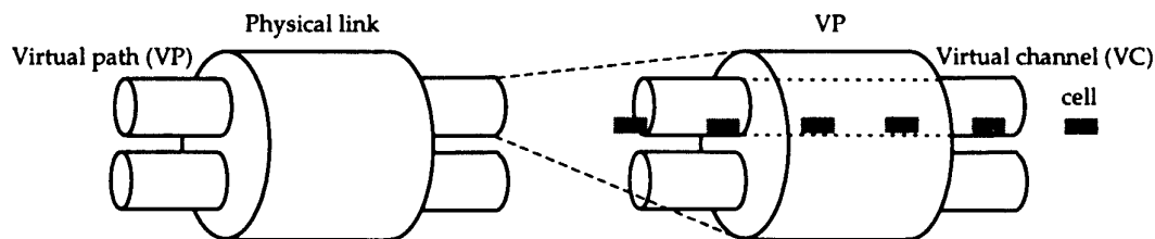
Figure 1: Physical Link, Virtual Path and Virtual Channel Relationship
