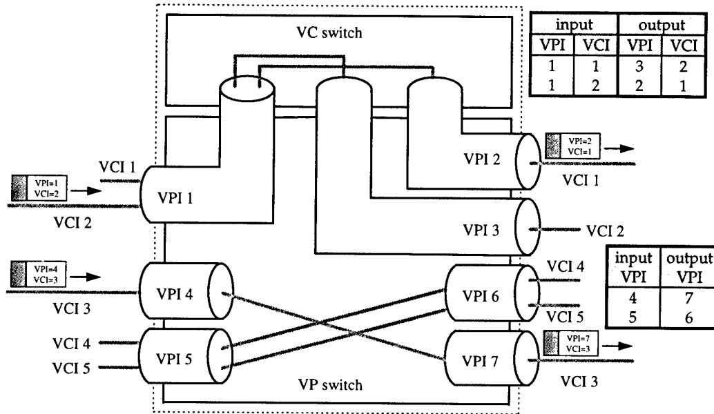
Figure 2: virtual channel and virtual path switching
