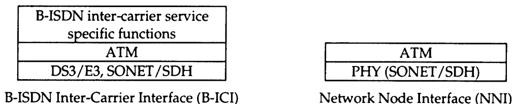
Figure 19 : Relation of a B-ICI to the NNI
