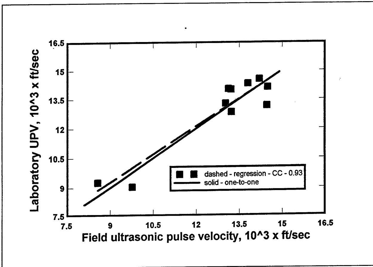
Figure 15. Correlation of average laboratory UPV and field UPV. (To convert feet to metres, multiply by in 0.3048)
