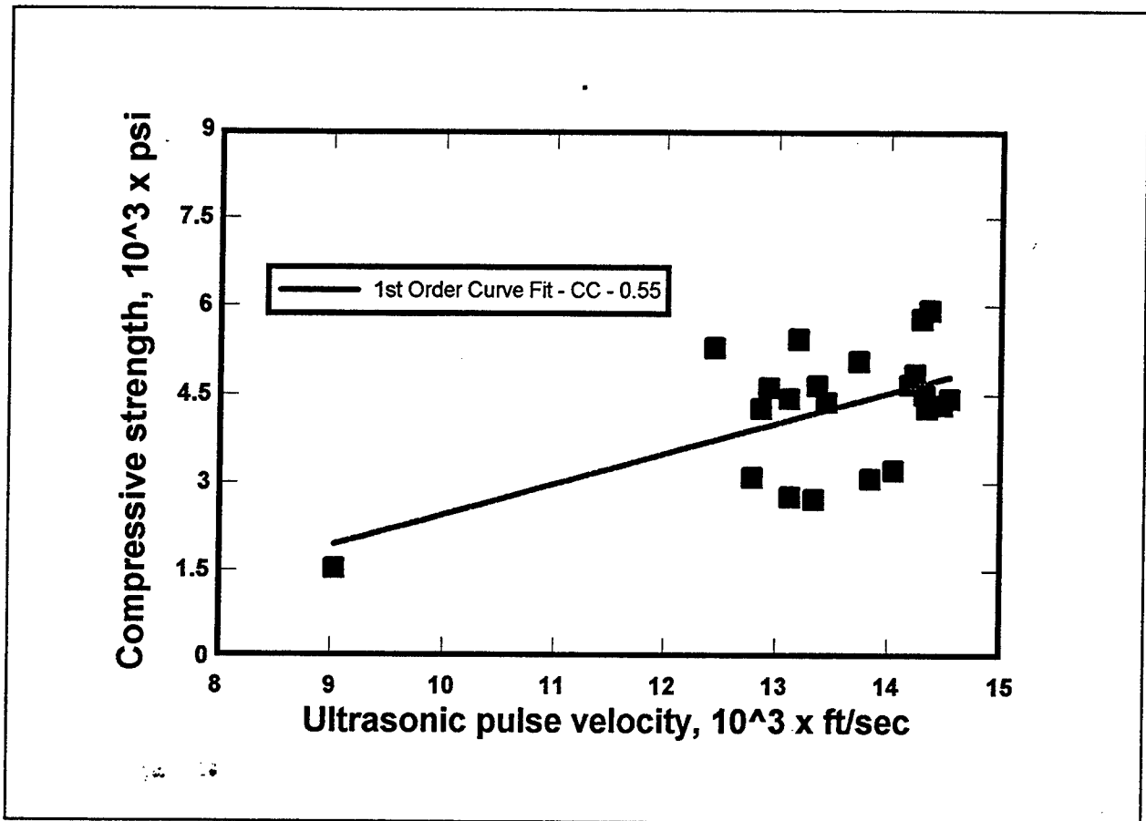
Figure 16. Correlation of individual core CS and laboratory UPV. (To convert pounds per square inch to megapascals, multiply by 0.006894757)
