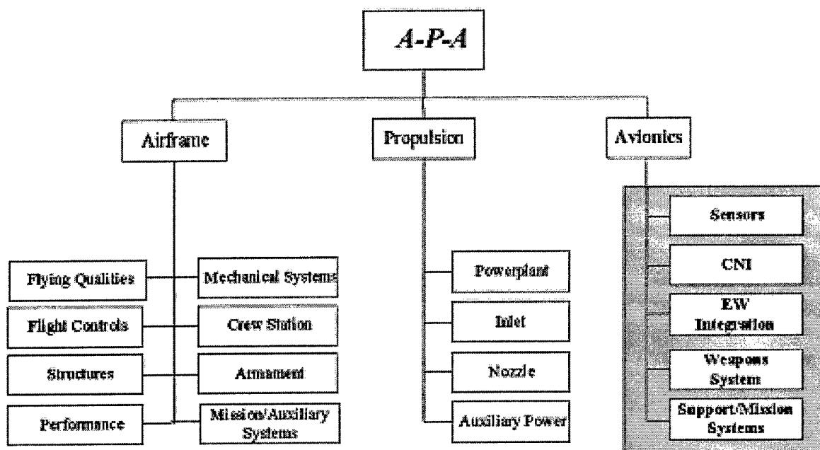
Figure 3.6. Avionics Disciplines/Systems.
