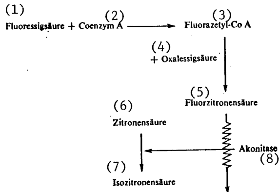
Figure 15.1. Inhibition of citric acid cycle by hydrofluoric acetic acid. Key: 1--Hydrofluoric acetic acid; 2--Coenzyme A; 3--Fluoroacetyl-Co A; 4--Ox- alacetic acid; 5--Hydrofluoric citric acid; 6--Citric acid; 7--Isocitric acid; 8--Aconitase.
