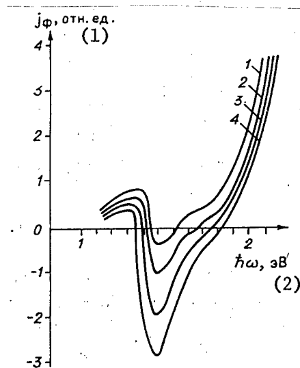
Figure 3. Spectral Distribution of Photocurrent of Structure with x = 0.3 at Different Bias Voltages U , V : 1-- -1.0 ; 2-- -0.5 ; 3-- 0 ; 4-- +2 .
