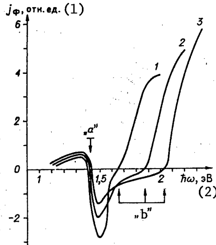
Figure 1. Spectral Distribution of Photocurrent j_f with Zero Bias of \text{M}-n^+\text{Al}_x\text{Ga}_{1-x}\text{As}-n\text{GaAs} Structures with Different Molar Fraction of Aluminum x : 1--0.2; 2--0.4; 3--0.7
