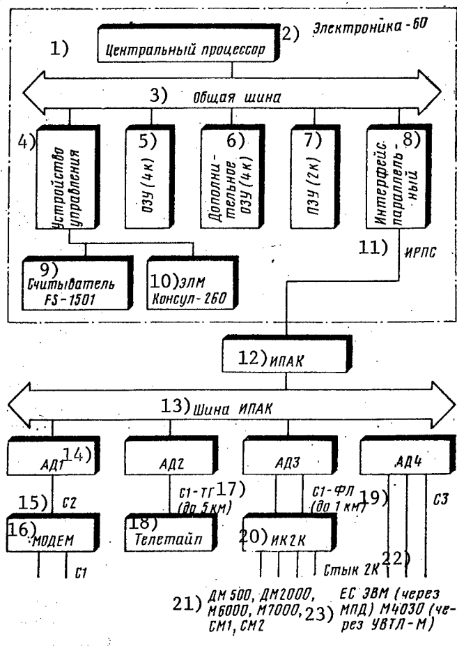
Figure 1. Structural Diagram of Terminal Concentrator Based on UVTK-KI Equipment
