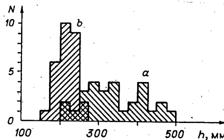
Figure 7. Histograms of Depths of Etching: a--without exposure control; b--with exposure control
