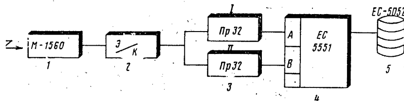
Figure 1. Structural Diagram of VK-32 Computer Complex: 1--"Minsk-1560" unit; 2--electronic switch; 3--"Minsk-32" processor; 4--YeS-5551 disk storage control unit (UU NMD); 5--YeS-5052 magnetic disks
