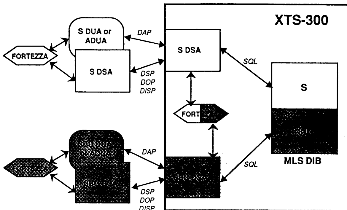
Figure 3.2. MLS Directory Server Components and Data Flows
