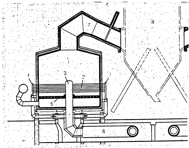
Figure 2: The fluidized-bed furnace, consisting of: Fluidized-bed combustion chamber (1), immersion heating surface (2), inner header (3), outer header (4), nozzle bottom (5), coaxial line (6), off-gas channel (7), and steam generator (8).
