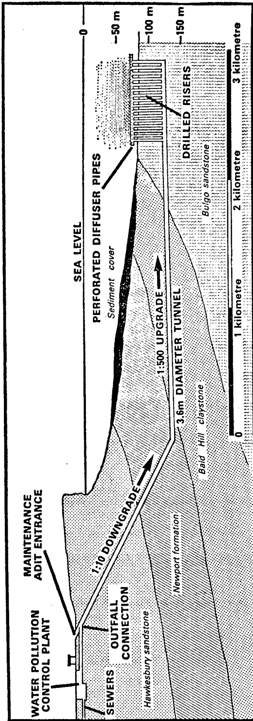
A cross-section of the construction work facing engineers.
