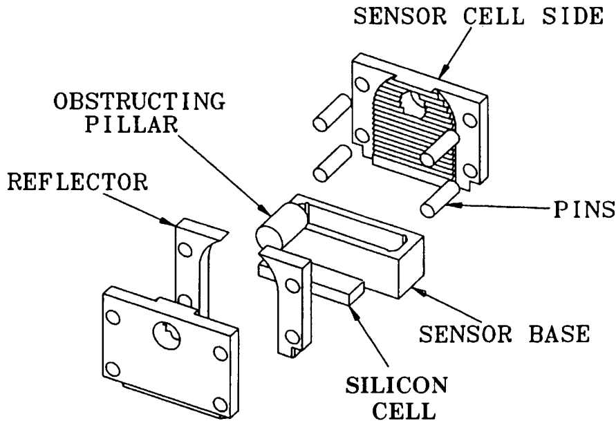
Figure 2. Assembly View of Prototype Sensor.
