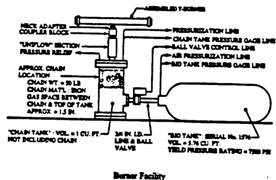
Fig. 7 T-burner test apparatus used in this study.
