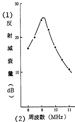
Figure 10. Example of Characteristic of an Antireflective Microwave Absorber Using Composite Ferrite
