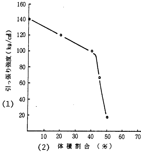
Figure 6. Tensile Strength of Composite Ferrite Formed by Mixing and Diffusing Mn-Zn Ferrite in Chloroprene Rubber
