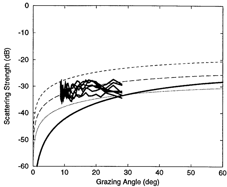
Fig. 7 — Bottom backscattering strength as a function of grazing angle at 1500,2000,2500,3000,3500,4000, and 4500 Hz during LWAD 98-2 scattering run 2. The source was at a depth of 70 m. The BSS values fall between the curves -20 + 10 \log(\sin \theta) and -30 + 10 \log(\sin \theta) .
