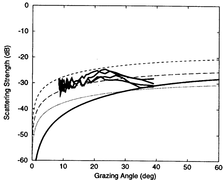
Fig. 6 — Bottom backscattering strength as a function of grazing angle at 2000,2500,3000 and 3500 Hz during LWAD 98-2 scattering run 2. The BSS curves are the averaged scattering strength curves shown in figures 2-5.
