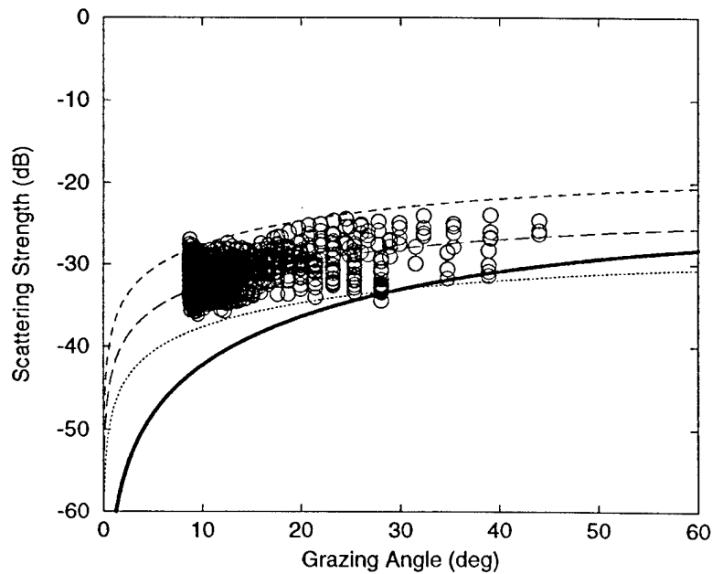
Fig. 8 — Bottom backscattering strength as a function of grazing angle at 1500,2000,2500,3000,3500,4000, and 4500 Hz for scattering runs 1 and 2. The BSS values (represented as circles) fall between the curves -20 + 10 \log(\sin \theta) and -30 + 10 \log(\sin \theta) .
