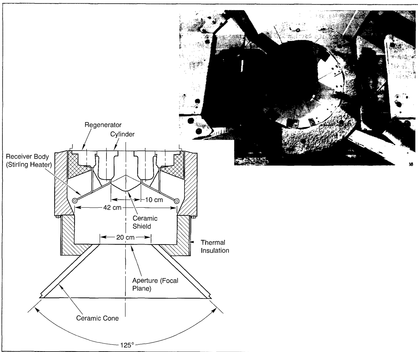
Figure 6-1a. Vanguard I receiver. Note water-cooled aperture protection shutters on either side.
