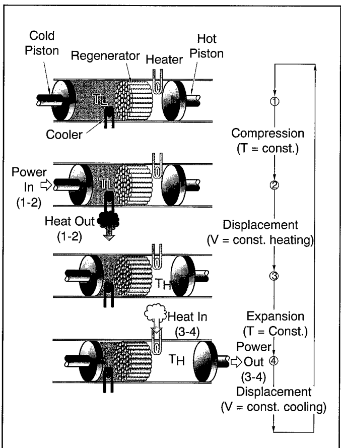
Figure 3-4. Basic processes of a kinematic Stirling engine. (Numbers refer to states in Figure 3-3.)
