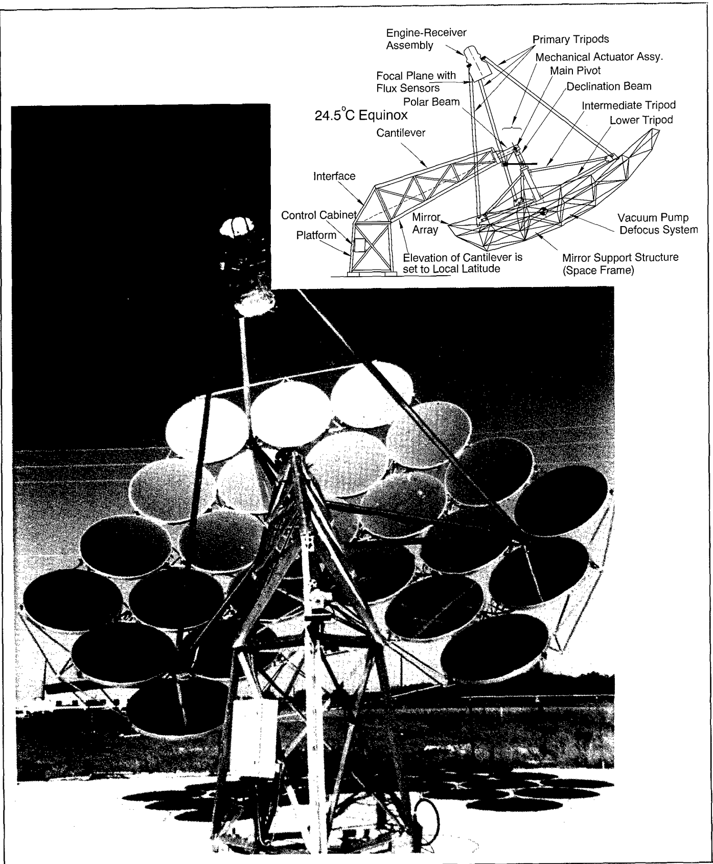
Figure 5-9. Cummins Power Generation CPG-460 multifaceted concentrator.
