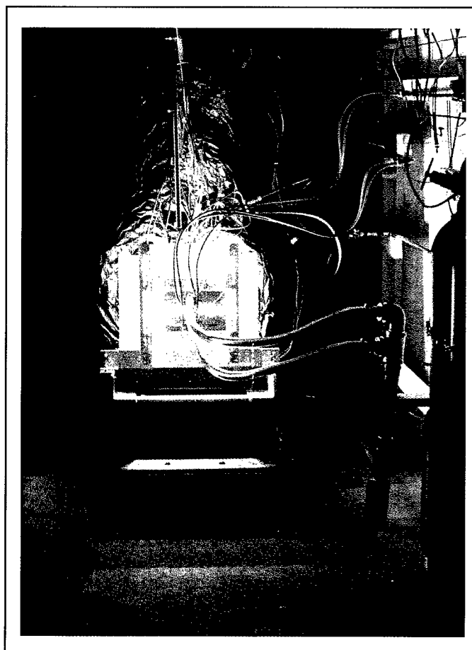
Figure 4-5. Stirling Technology hybrid receiver in a test cell using radiant lamp solar simulation.
