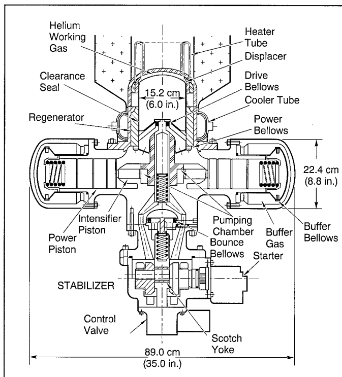
Figure 4-4. The Stirling Technology Corporation STIRLIC™ 25-kW engine.
