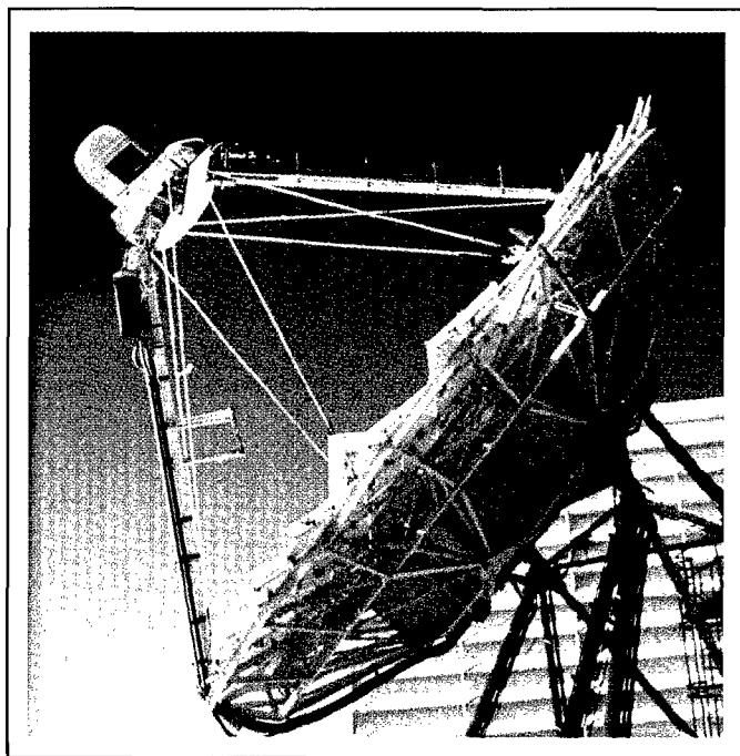
Figure 2-6. Stirling Thermal Motors 25-kW e solar power conversion system package under test at Sandia National Laboratories.
