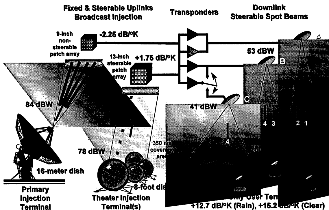
Figure 3 GBS Phase Two Space Segment [Ref. 3]
