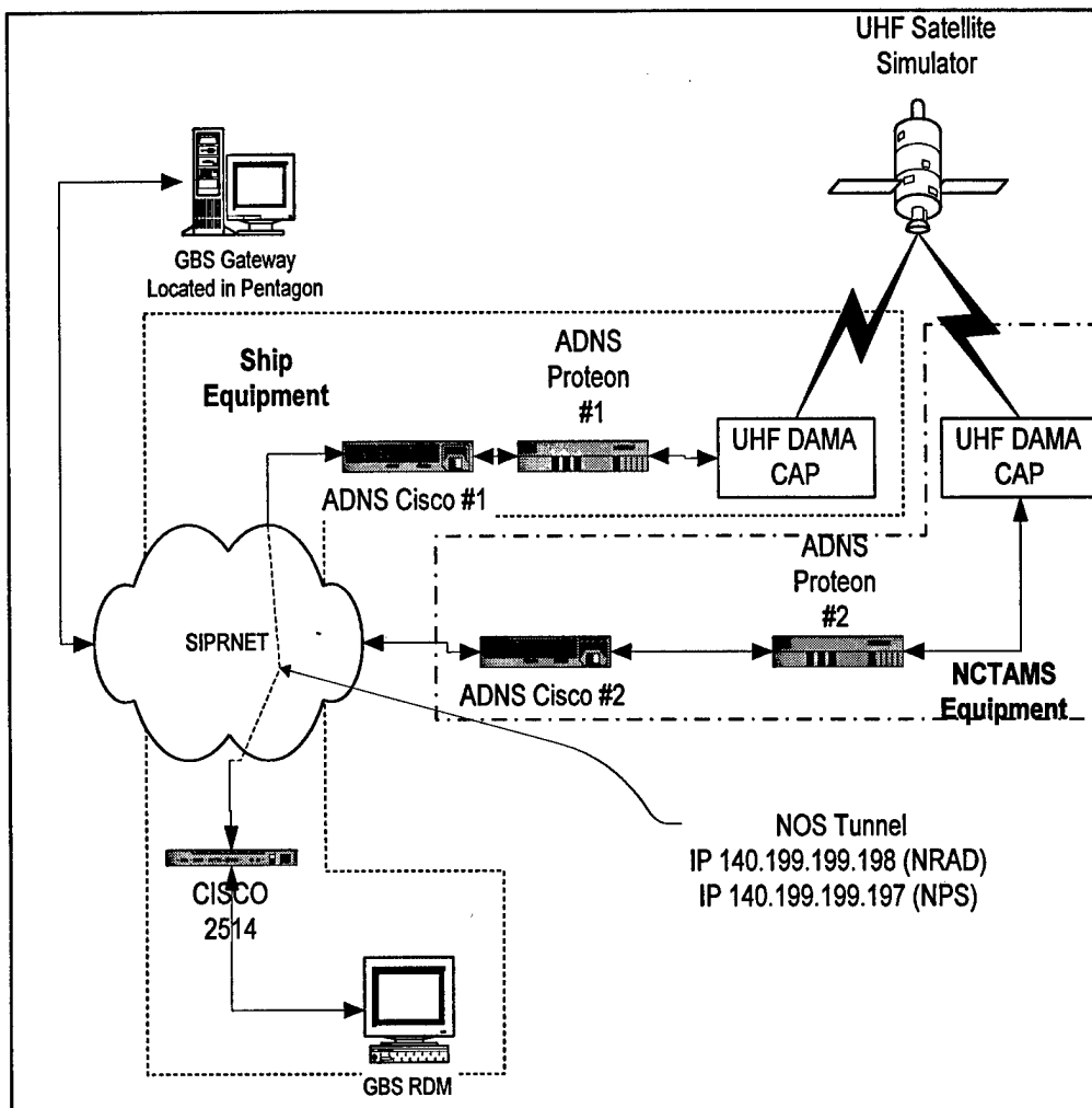
Figure 11 Tunneling Setup
