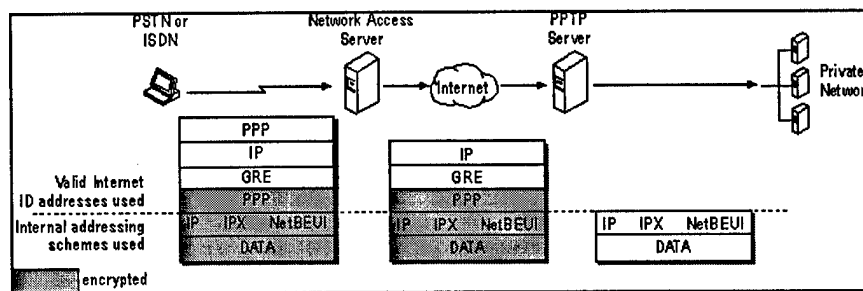
Figure 4 PPTP Connection
