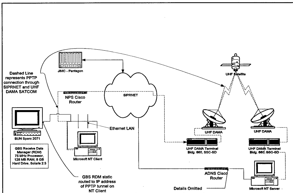
Figure 16 PPTP Tunnel
