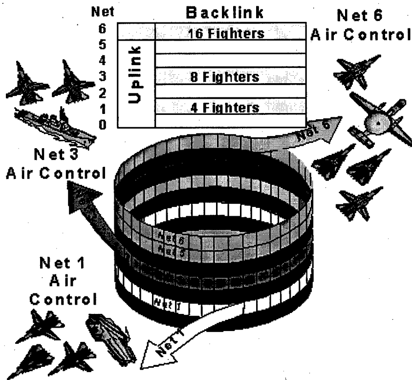
Figure 4.7 Stacking Nets
