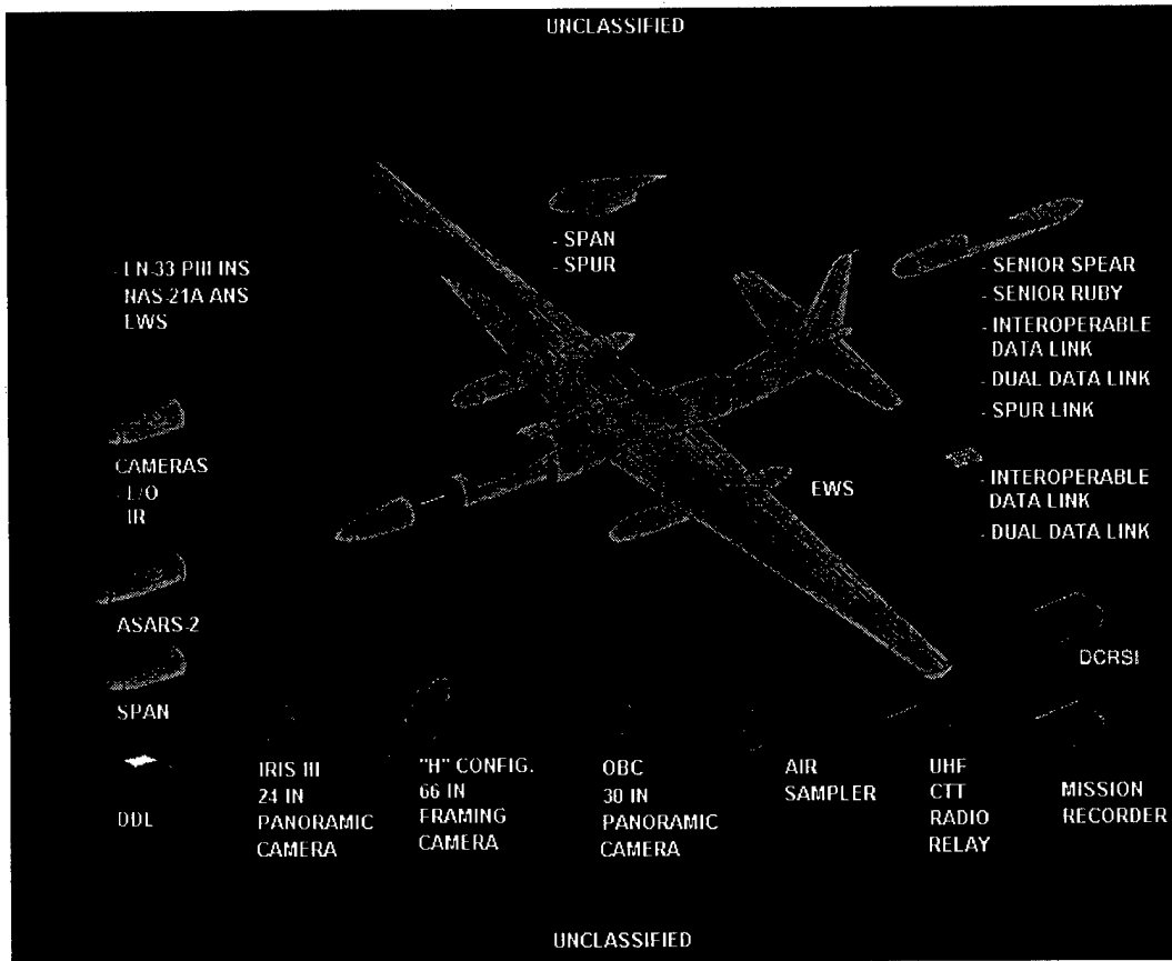
Figure 4.2 U-2 Payload
