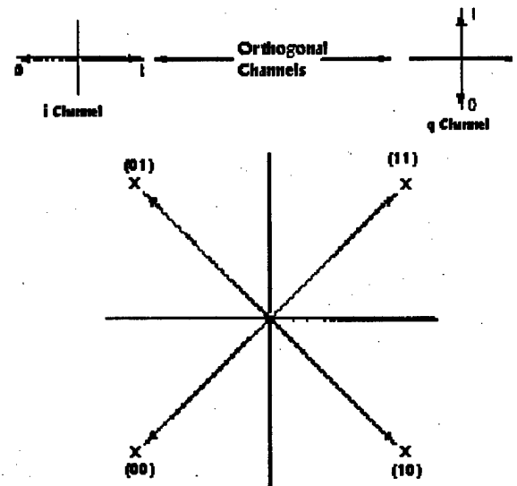
Figure 4.4 State Generation in QPSK
