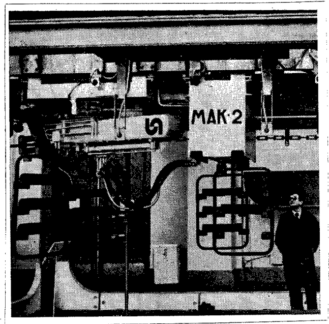
Figure 4. VNIPTmash's MAK-2-320 automatic conveyor manipulator.
