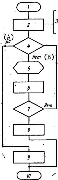
Figure 4. Block diagram of algorithm for recovering task file address: A - YES; B - NO; 1 - initialization; 2 - preparation; 3 - recovery of \bar{S}_z address, counter i (i: = n); 4 - |S_{rei} - S_{zi}| \leq \epsilon_i ?; 5 - readdress file S_z ; 6 - decrease i: i-1; 7 - i = 0; 8 - IRO: =1; 9 - IRO: =0; 10 - output.
