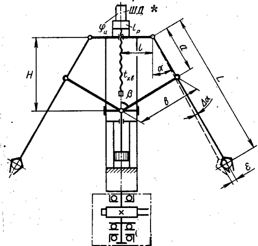
Figure 3. Kinematic diagram of mod. SPM-MPI automatic manipulator. * - stepper motor.
