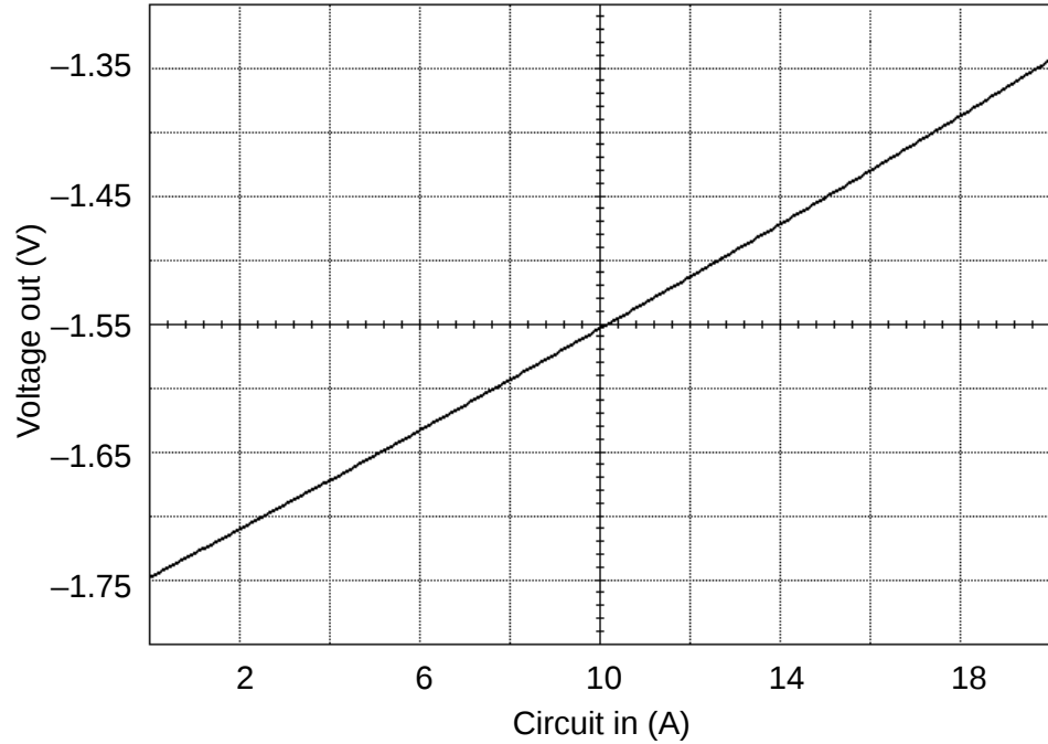
Figure 7. Result of SPICE simulation for amplifier.
