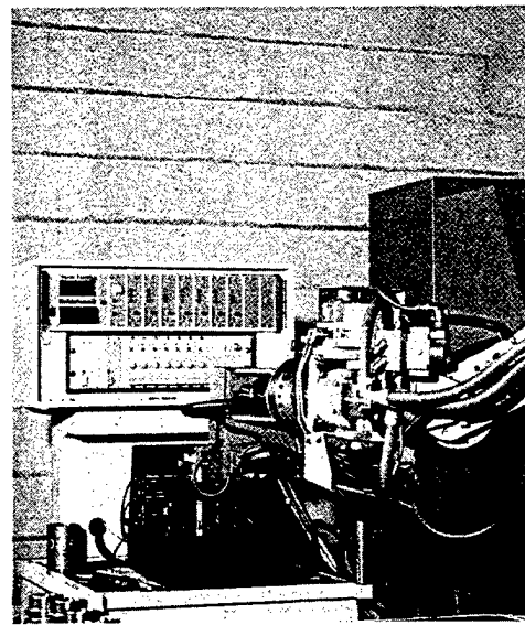
Electronic control and analysis of measurements for tool correction.
