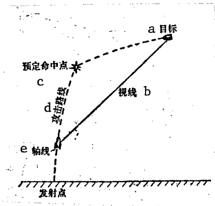
Fig. 4.3. Intercept path
