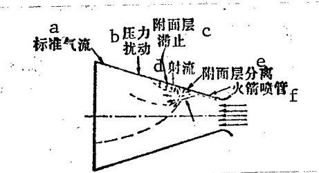
Fig. 5.5. Secondary nozzle thrust vector control
