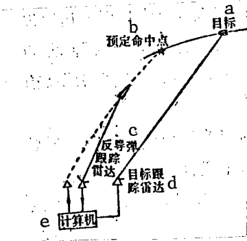
Fig. 4.1. Head-on intercept
