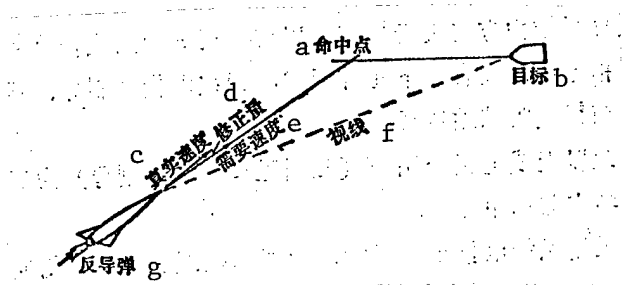
Fig. 4.9. Command guidance
