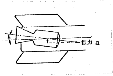
Fig. 4.7. Swiveled engine
