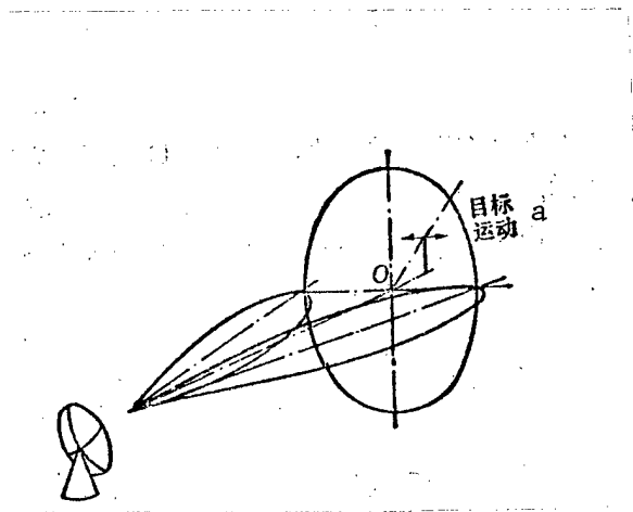
Fig. 7.13. Conical-scan radar
