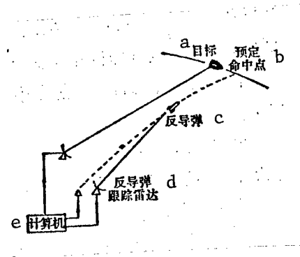
Fig. 4.2. Rear intercept
