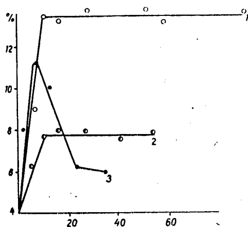
Yield of chromosome aberrations as a function of dosage of laser radiation.
