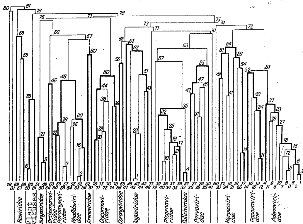
Figure 2. Dendrogram illustrating the process of successive combination of different viruses into groups when missing data are replaced with a random figure
