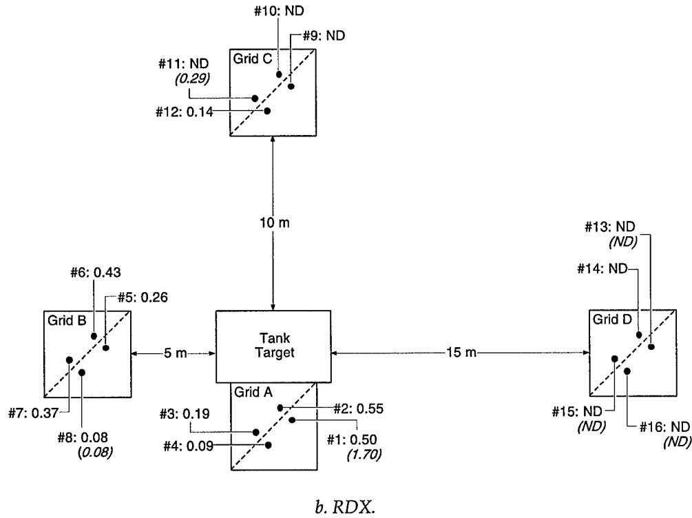
Figure 8. Areal distribution of explosives residues (mg/kg) in surface soils for sampling location 1-44 (duplicate samples italic and in parentheses).
