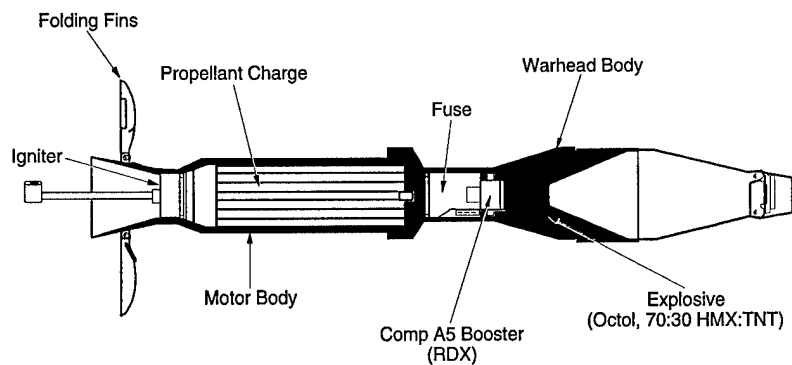
Figure 4. 66-mm M72 LAW rocket.
