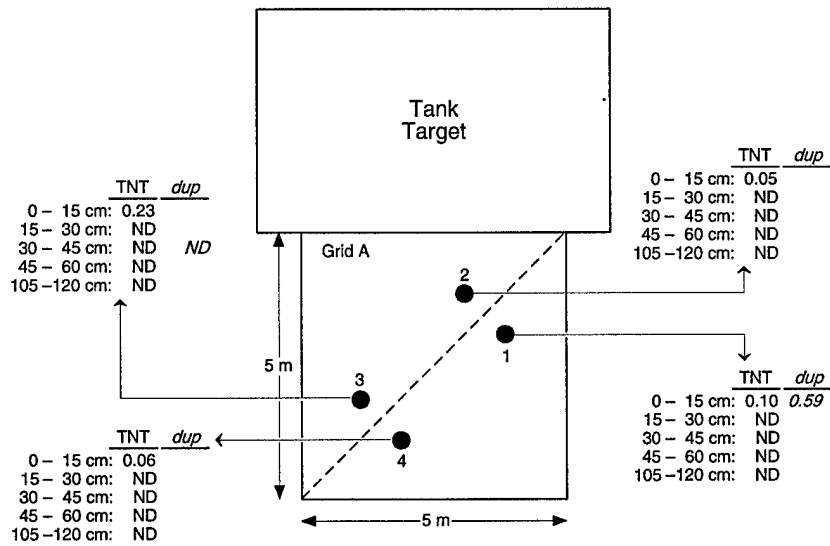
Figure 7. Concentrations (mg/kg) of explosives residues as a function of depth for grid A, sampling location 1-44.
