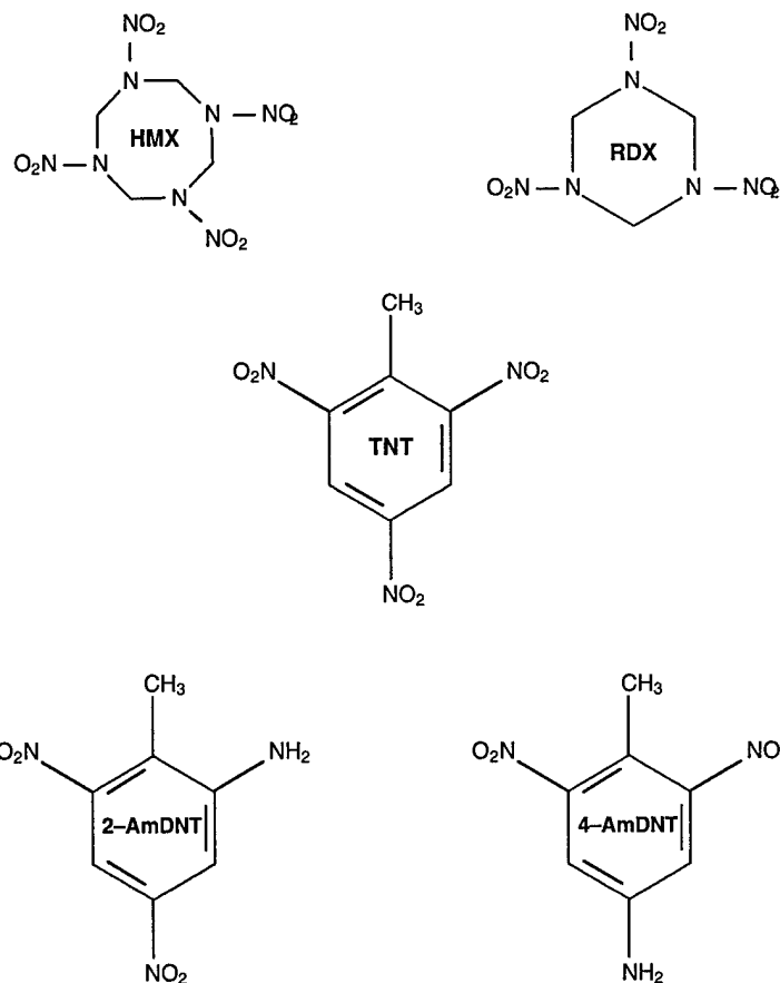
Figure 1. Structures of explosives detected at the Fort Ord inland firing ranges.
