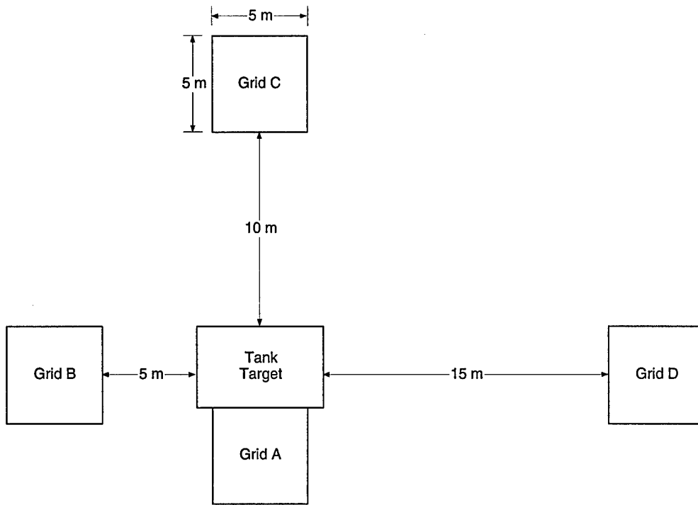
Figure 5. Sampling grids for area 1-44.
