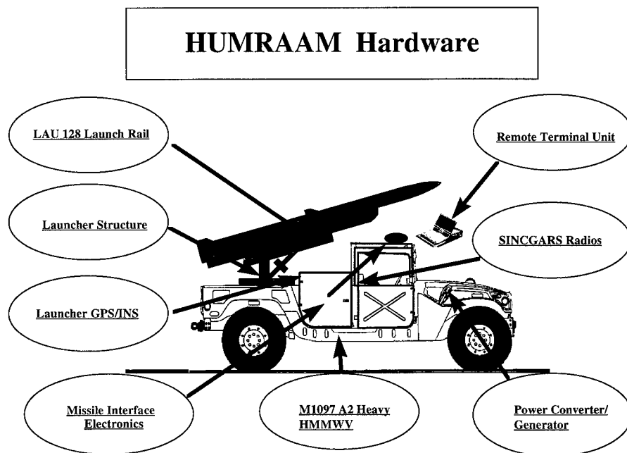
Figure 3. HUMRAAM launcher major functional elements.
