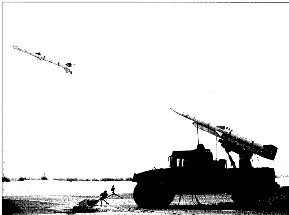
Figure 4. HUMRAAM ballistic test firing at Eglin Air Force Base, FL.
