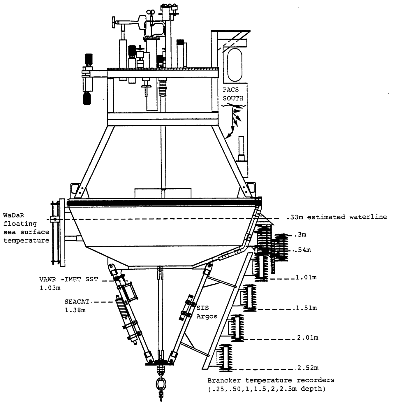
Figure 8: PACS 1 South discus buoy with tower and bridle instrumentation.
