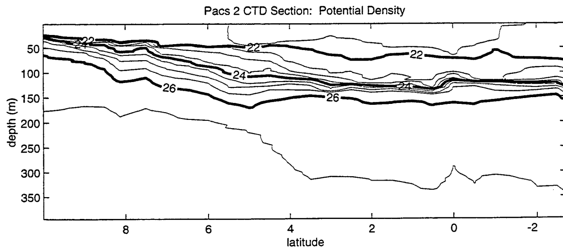
Figure A2-2: Composite plot of CTD data taken during TN 073.
