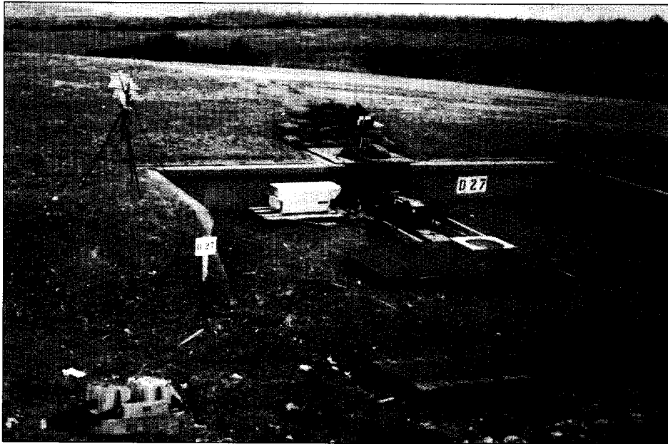
LASS system installed on Target Board Range 301, Grafenwoehr, Germany. The target board is in down position to show all LASS components.
