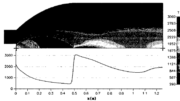
(c) Temperature Contours and Centerline Profile, (K)
