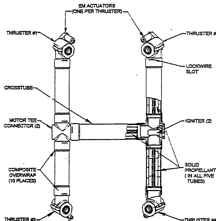
Figure 6-1. Aerojet's Pintle Escape Propulsion System (PEPS) (McDonnell Douglas, 1994)
