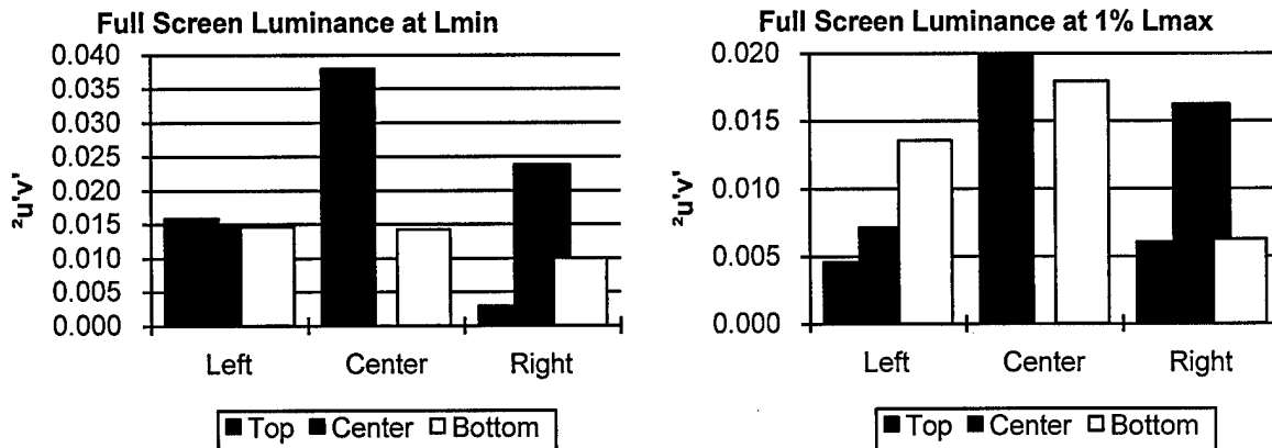
Fig. II.A-8 Spatial Uniformity of Chromaticity (vs. Center) A chromaticity error, z'u'v' , of 0.004 is visible.
