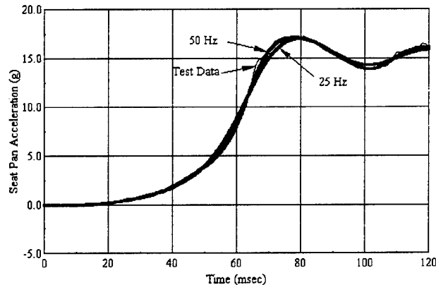
Figure 7. Ejection Seat Acceleration Filtered at 25 and 50 Hz
