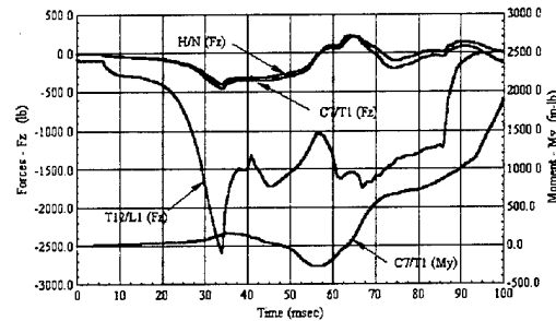
6B - Crashworthy Seat
