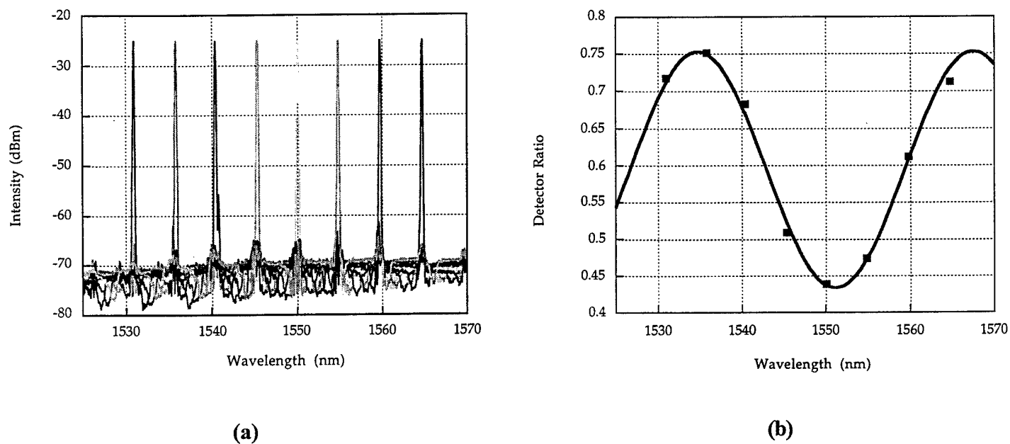
Figure 5. Wide range wavelength scan showing laser spectra (a) and wavelength monitor divided output ratio (b)
